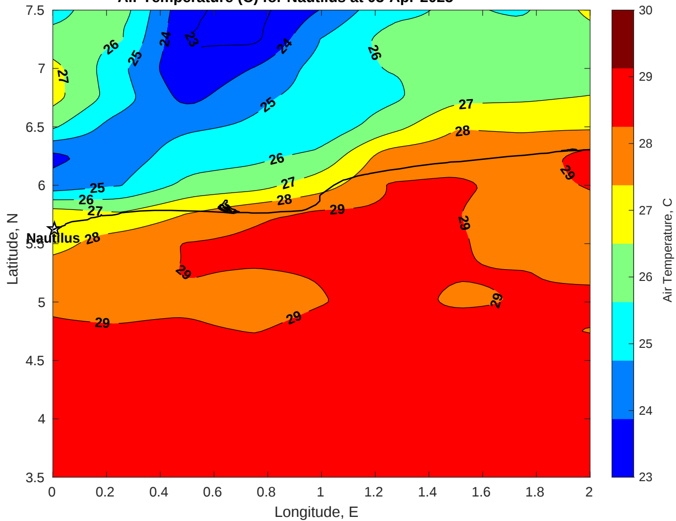
Air Temperature (C) for Nautilus at 03-Apr-2025
