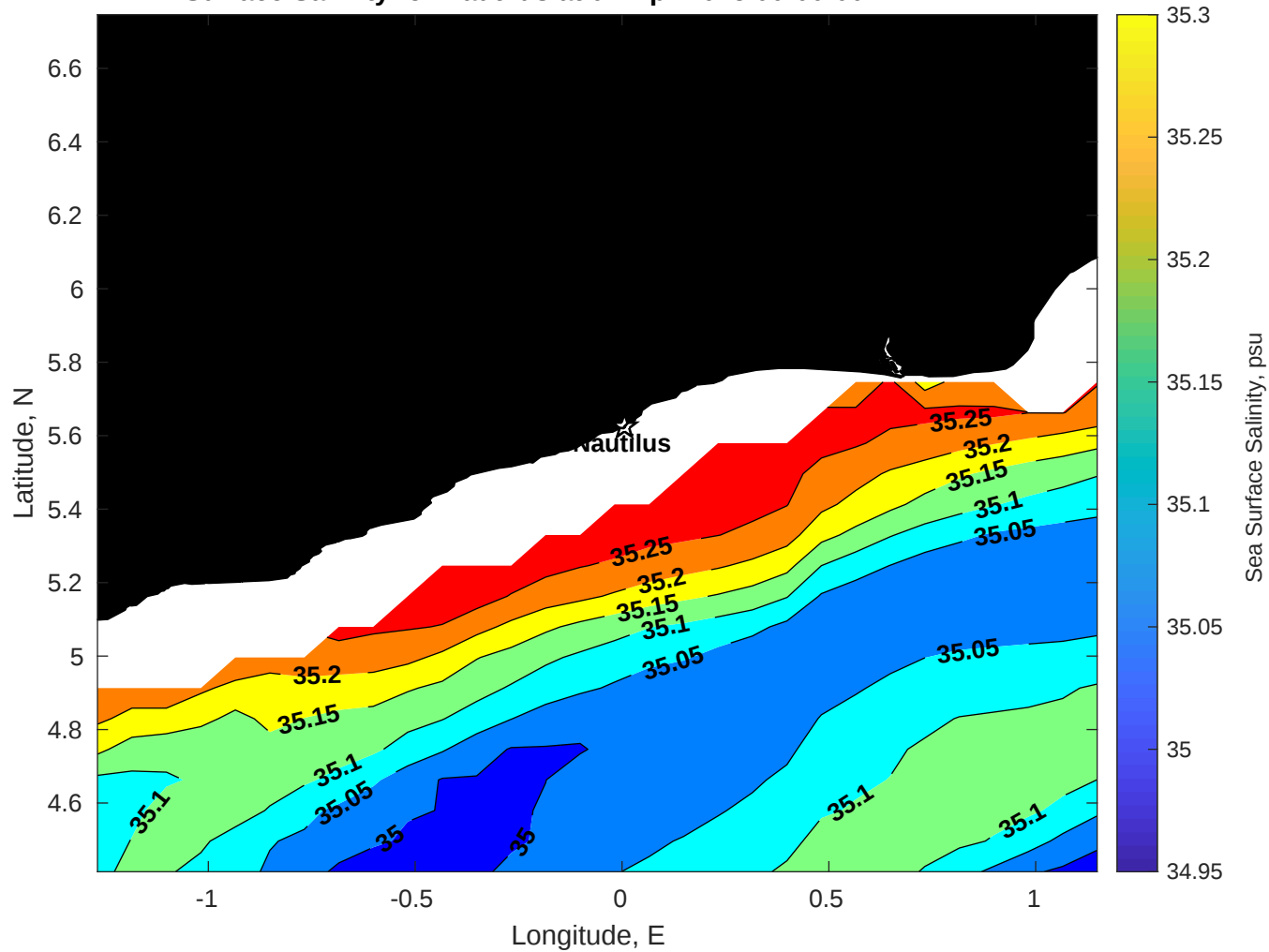
Surface Salinity for Nautilus at 02-Apr-2025 00:00:00
