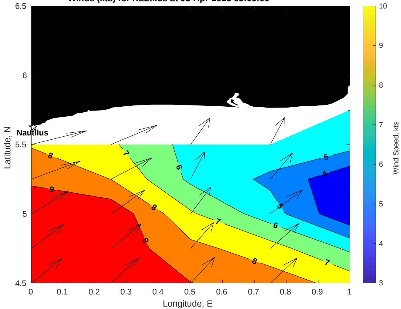
Winds (kts) for Nautilus at 03-Apr-2025 09:00:00
