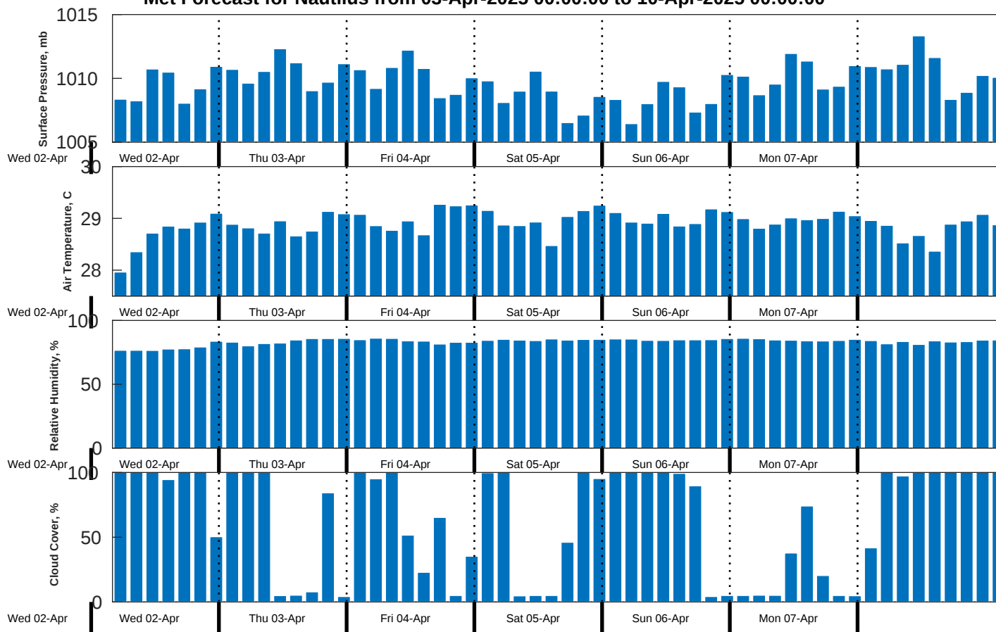
Met Forecast for Nautilus from 03-Apr-2025 00:00:00 to 10-Apr-2025 00:00:00
