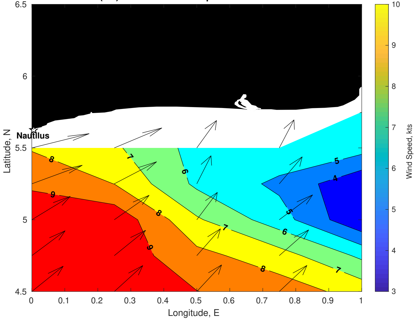
Winds (kts) for Nautilus at 03-Apr-2025 09:00:00
