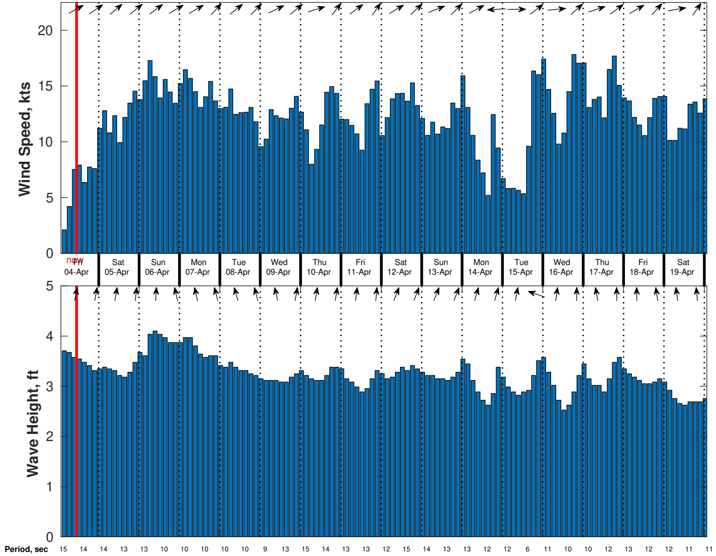
Wind & Wave Forecast for Nautilus from 03-Apr-2025 02:00:00 to 19-Apr-2025 02:00:00
