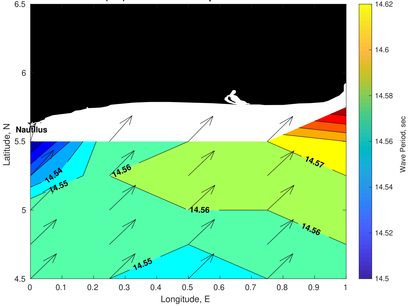
Wave Period (sec) for Nautilus at 03-Apr-2025 09:00:00
