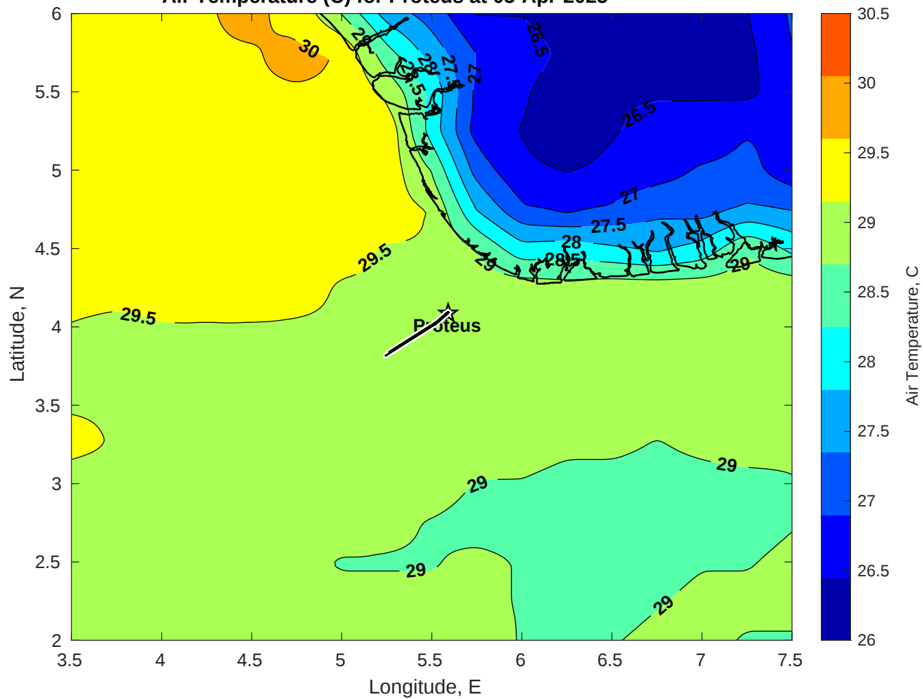
Air Temperature (C) for Proteus at 03-Apr-2025
