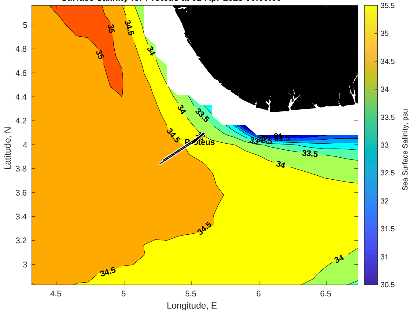
Surface Salinity for Proteus at 02-Apr-2025 00:00:00
