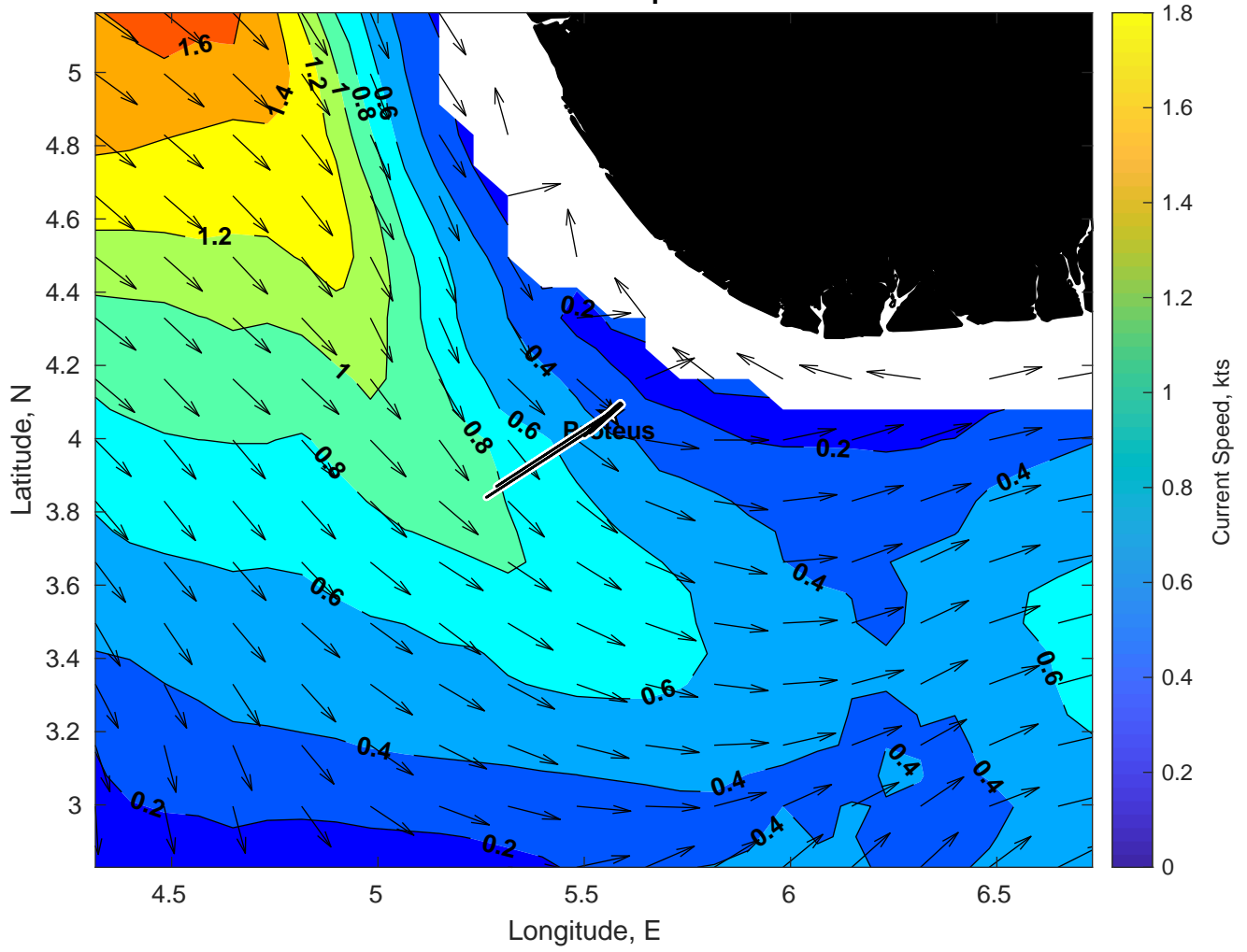
Surface Currents for Proteus at 02-Apr-2025 00:00:00
