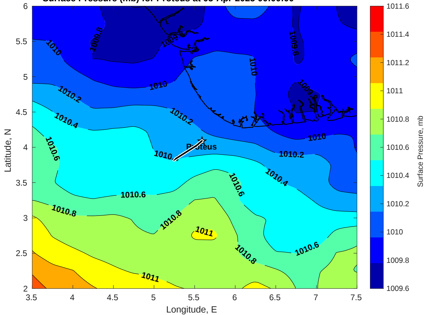
Surface Pressure (mb) for Proteus at 05-Apr-2025 00:00:00
