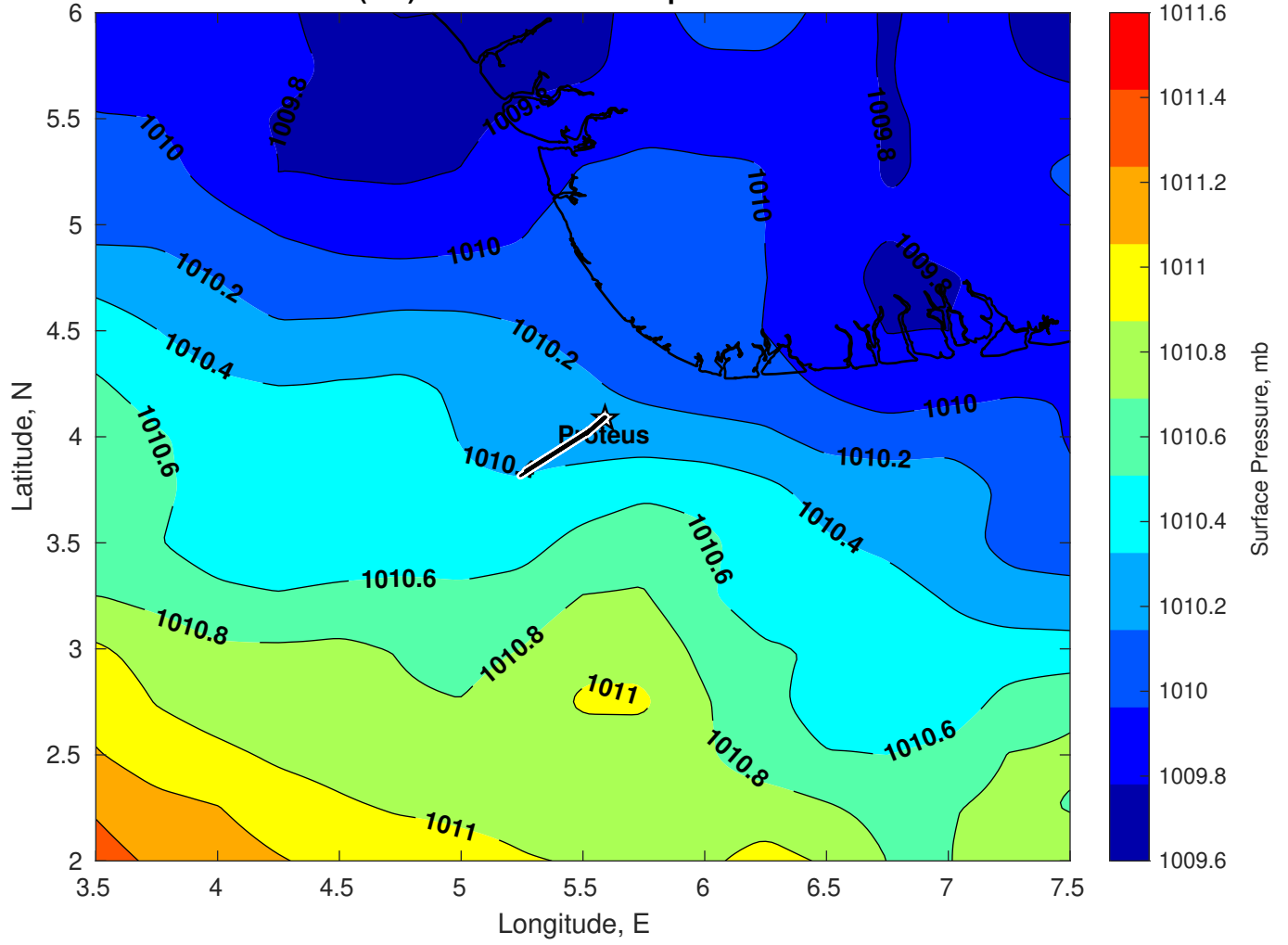
Surface Pressure (mb) for Proteus at 05-Apr-2025 00:00:00
