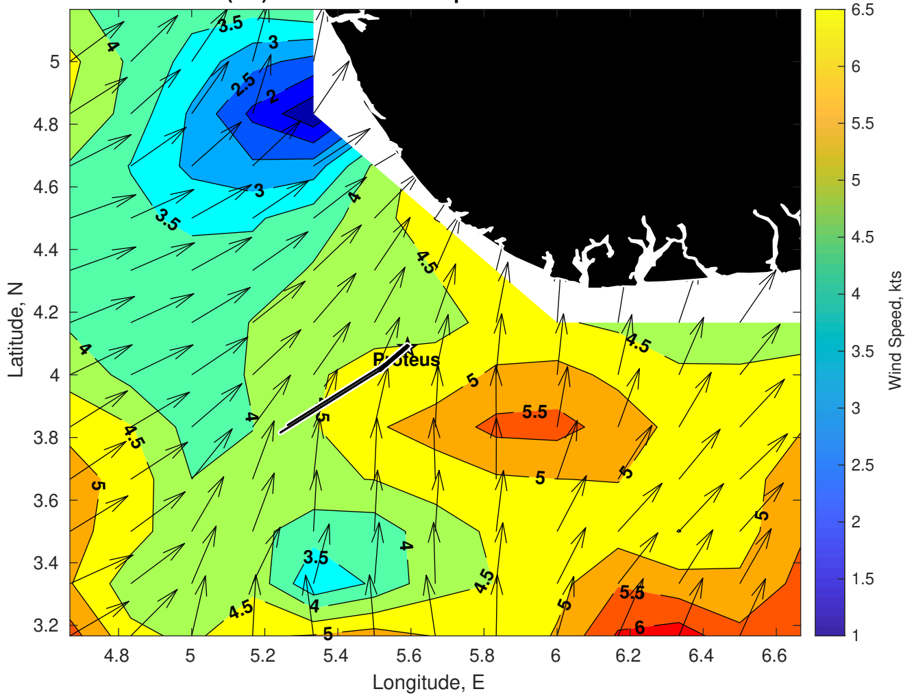
Winds (kts) for Proteus at 03-Apr-2025 09:00:00
