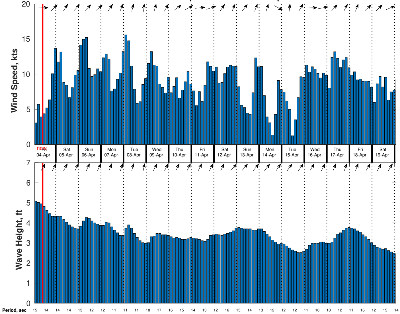
Wind & Wave Forecast for Proteus from 03-Apr-2025 01:00:00 to 19-Apr-2025 01:00:00
