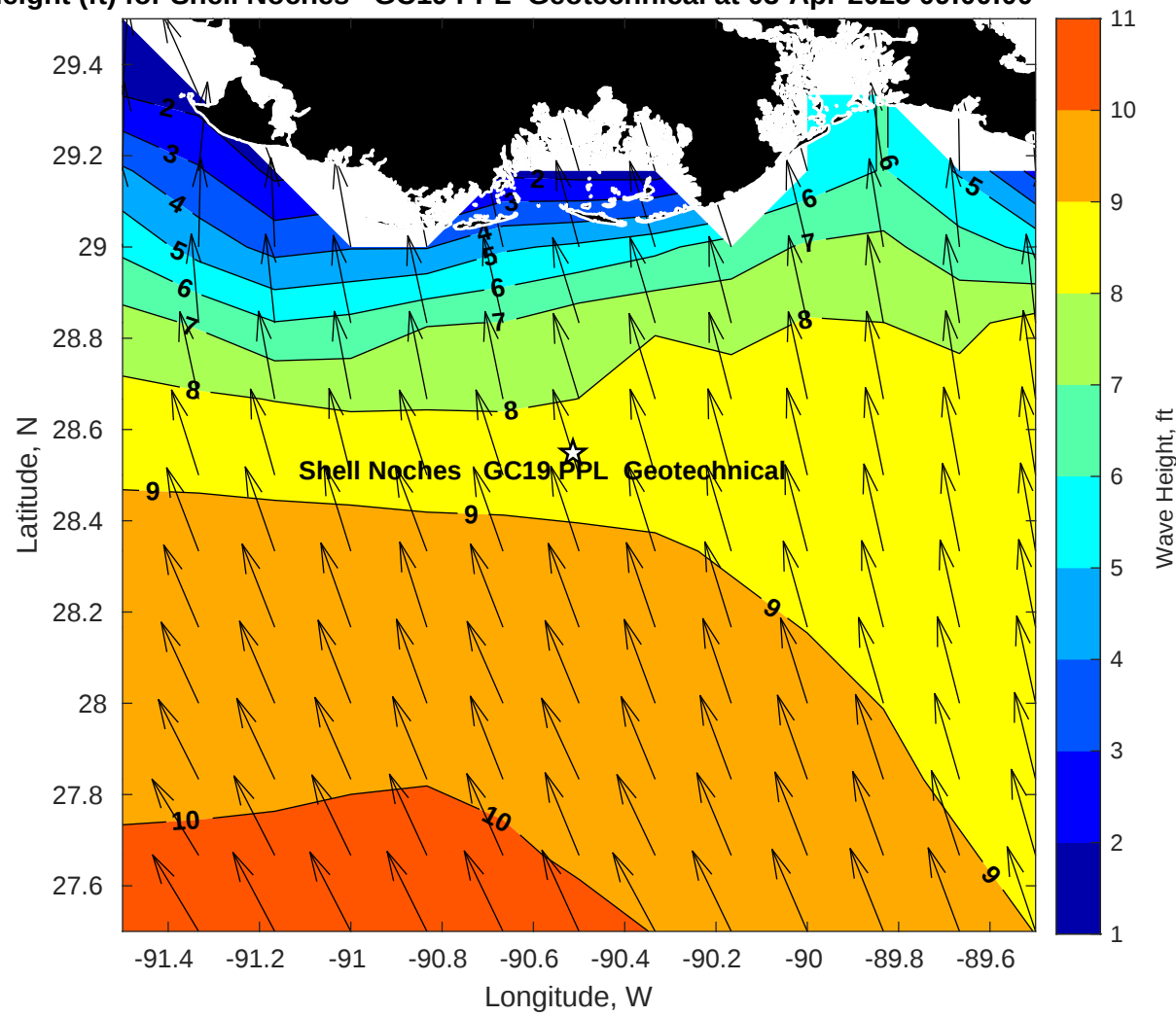
Wave Height (ft) for Shell Noches GC19 PPL Geotechnical at 03-Apr-2025 09:00:00
