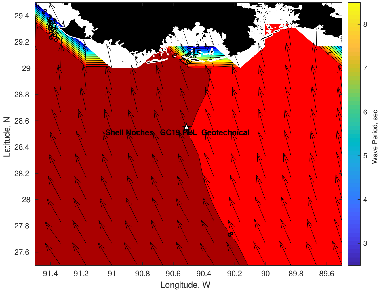
Wave Period (sec) for Shell Noches GC19 PPL Geotechnical at 03-Apr-2025 09:00:00
