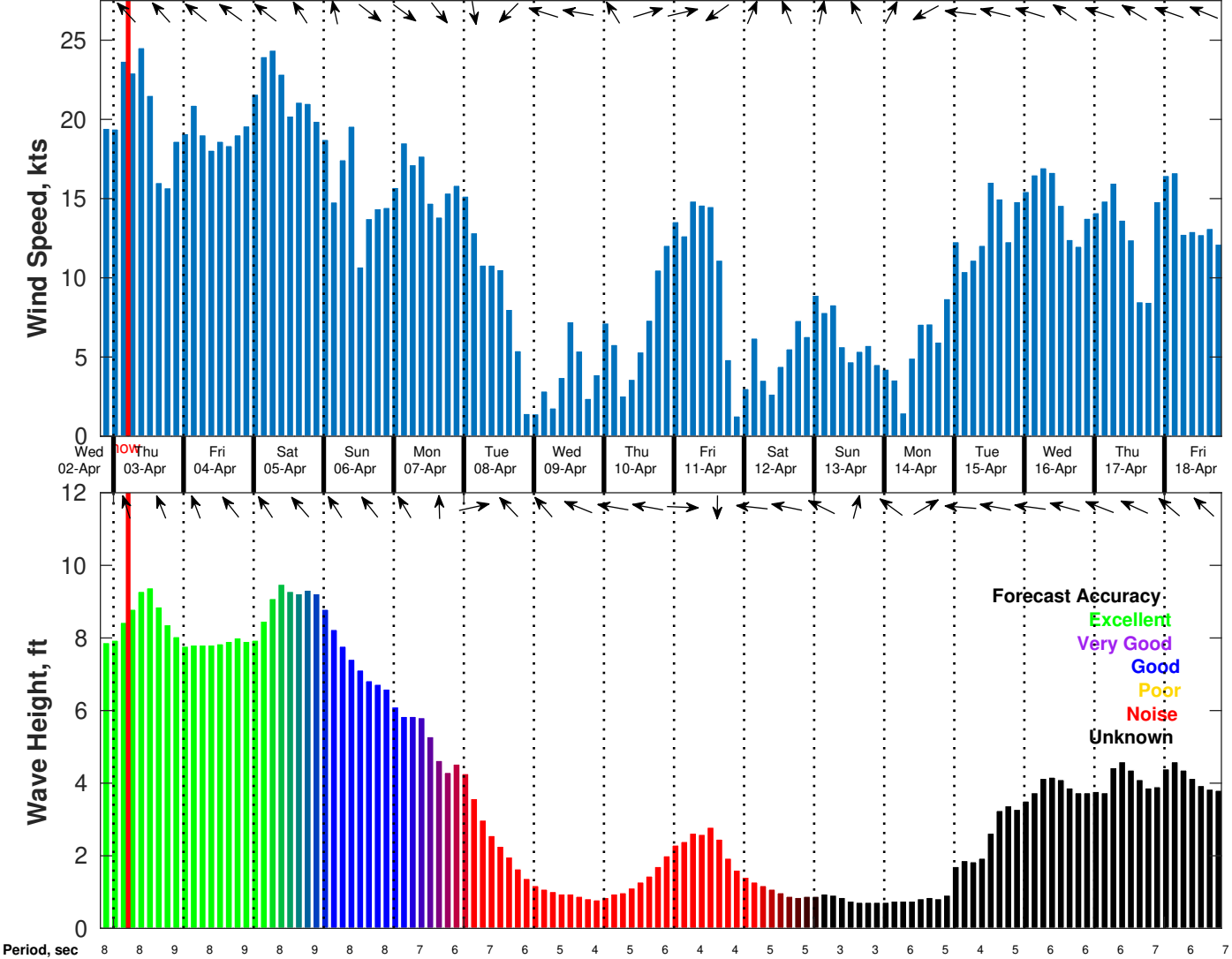
Wind & Wave Forecast for Shell Noches GC19 PPL Geotechnical from 02-Apr-2025 20:00:00 to 18-Apr-2025 20:00:00
