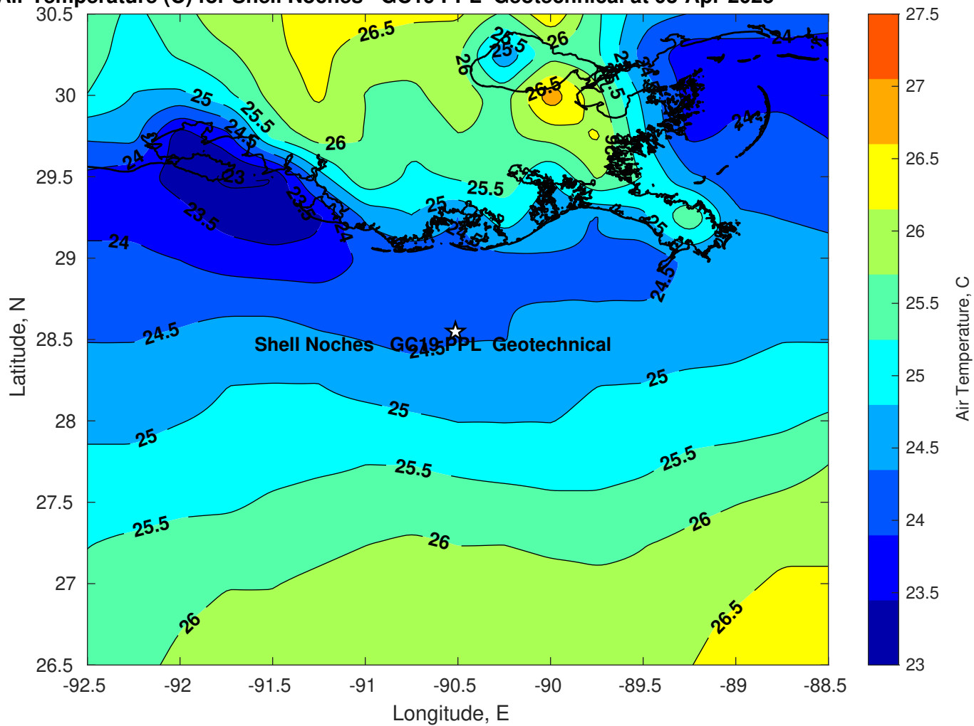
Air Temperature (C) for Shell Noches GC19 PPL Geotechnical at 03-Apr-2025
