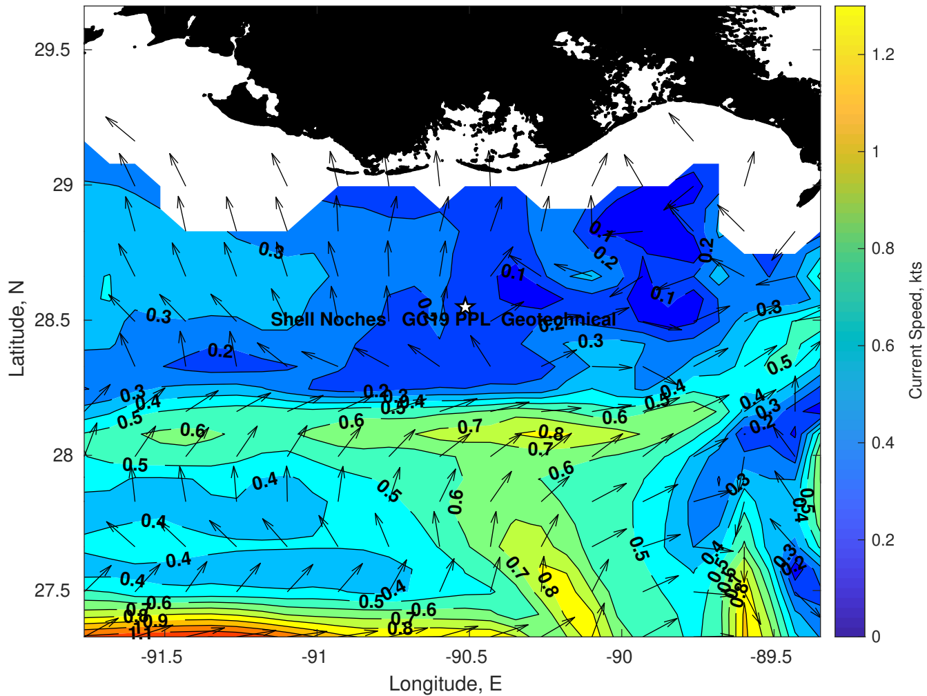
Surface Currents for Shell Noches GC19 PPL Geotechnical at 02-Apr-2025 00:00:00
