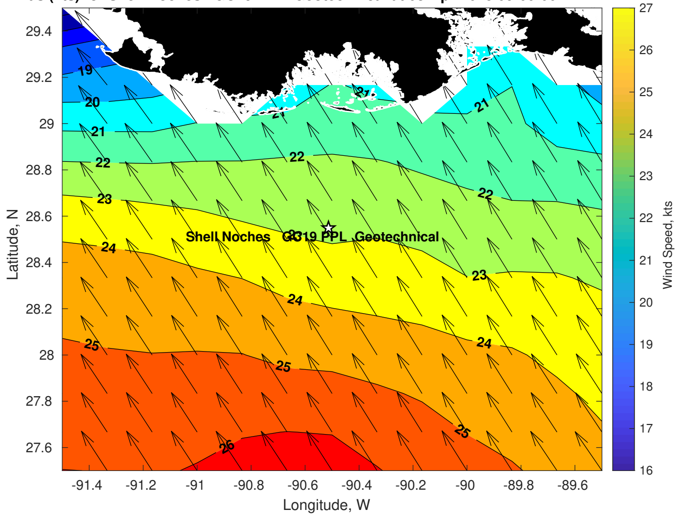
Winds (kts) for Shell Noches GC19 PPL Geotechnical at 03-Apr-2025 09:00:00
