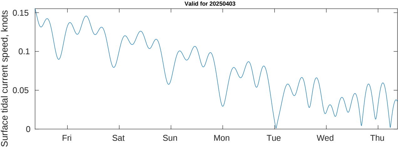
Tidal Currents and Heights for Shell Noches GC19 PPL Geotechnical at 20250403
