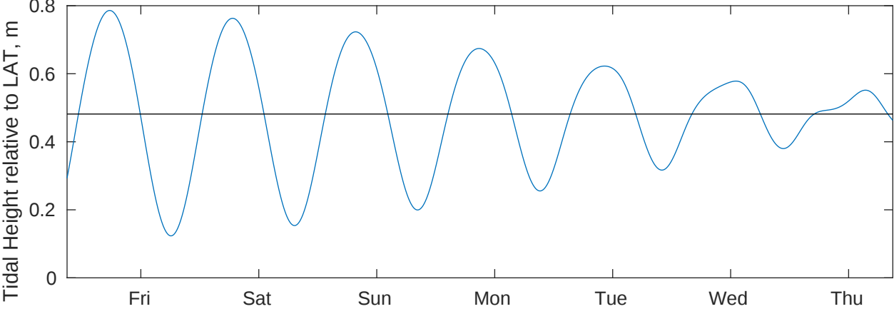
Tidal Currents and Heights for Shell Noches GC19 PPL Geotechnical at 20250403
