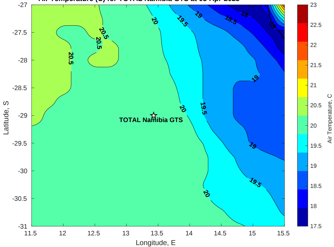
Air Temperature (C) for TOTAL Namibia GTS at 03-Apr-2025
