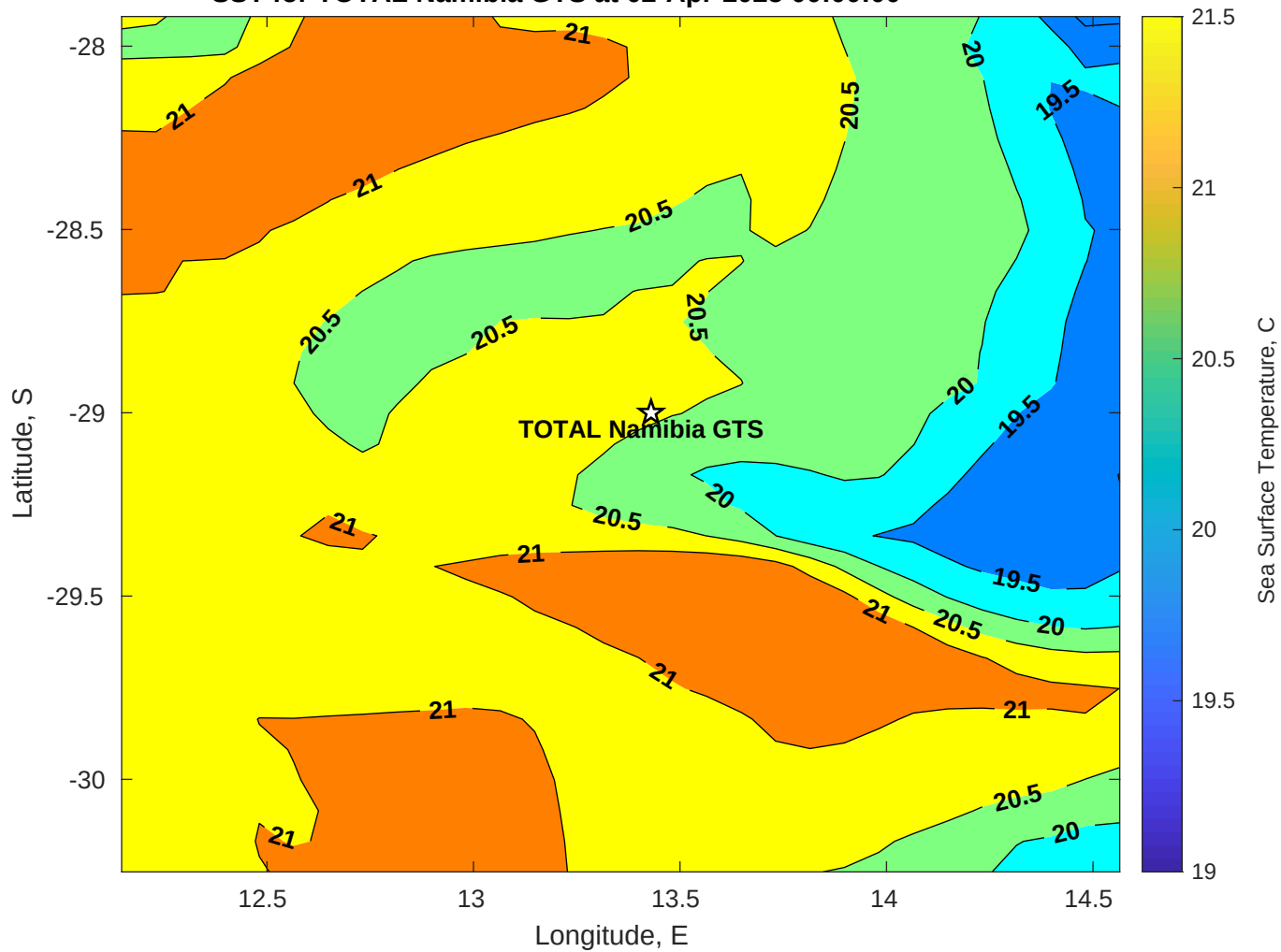
SST for TOTAL Namibia GTS at 02-Apr-2025 00:00:00
