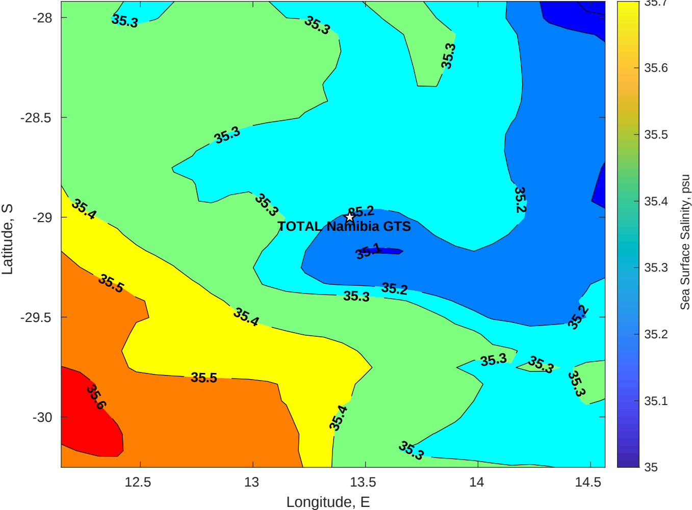
Surface Salinity for TOTAL Namibia GTS at 02-Apr-2025 00:00:00
