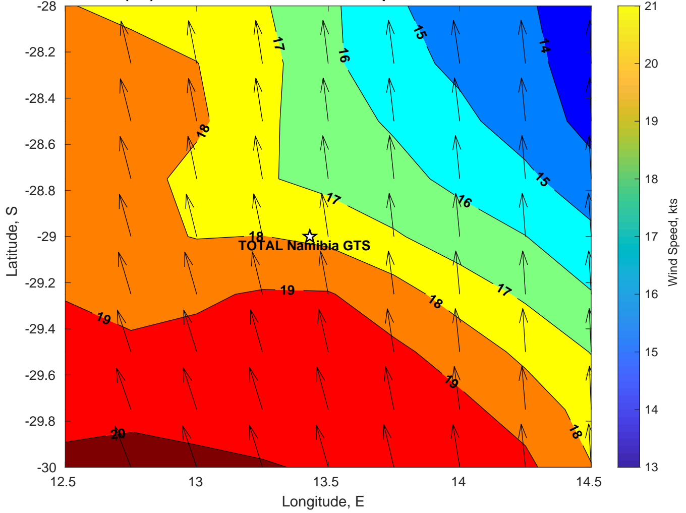
Winds (kts) for TOTAL Namibia GTS at 03-Apr-2025 09:00:00
