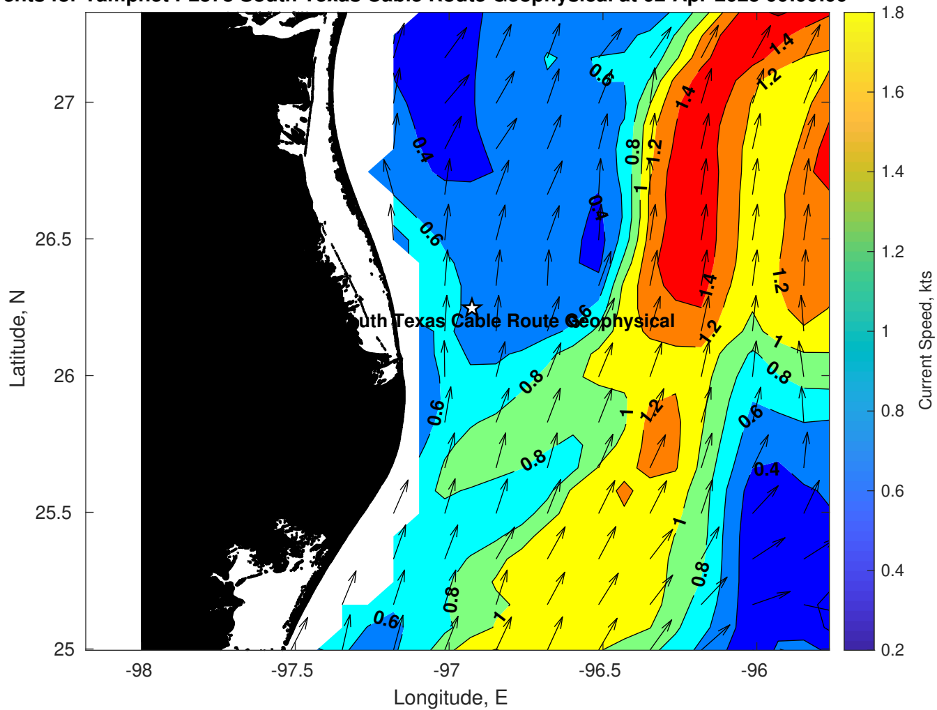
Surface Currents for Tampnet P2378 South Texas Cable Route Geophysical at 02-Apr-2025 00:00:00
