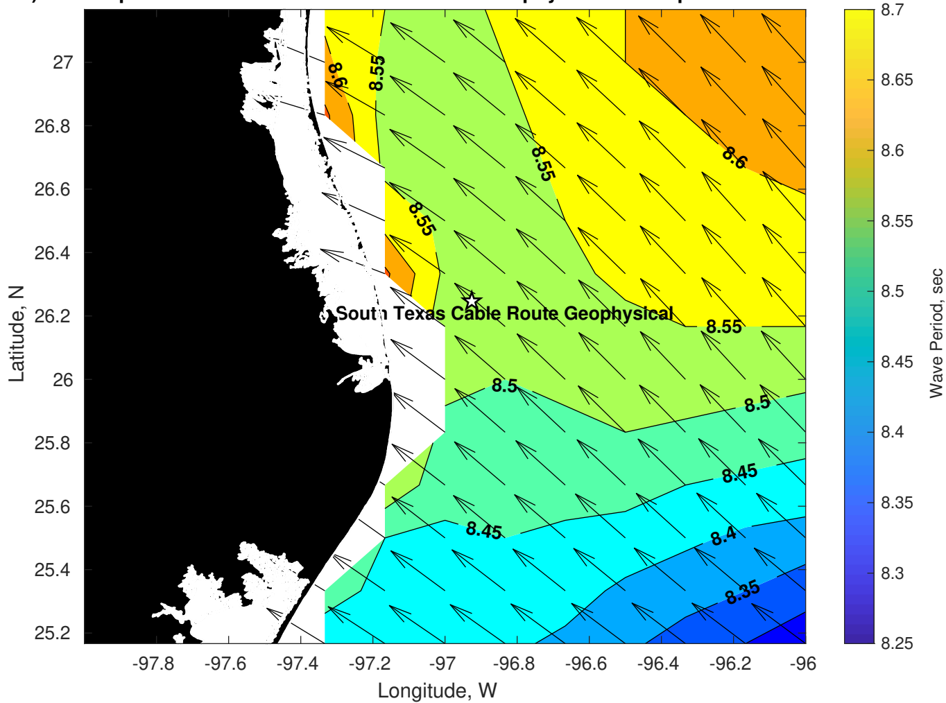
Period (sec) for Tampnet P2378 South Texas Cable Route Geophysical at 03-Apr-2025 09:00:00
