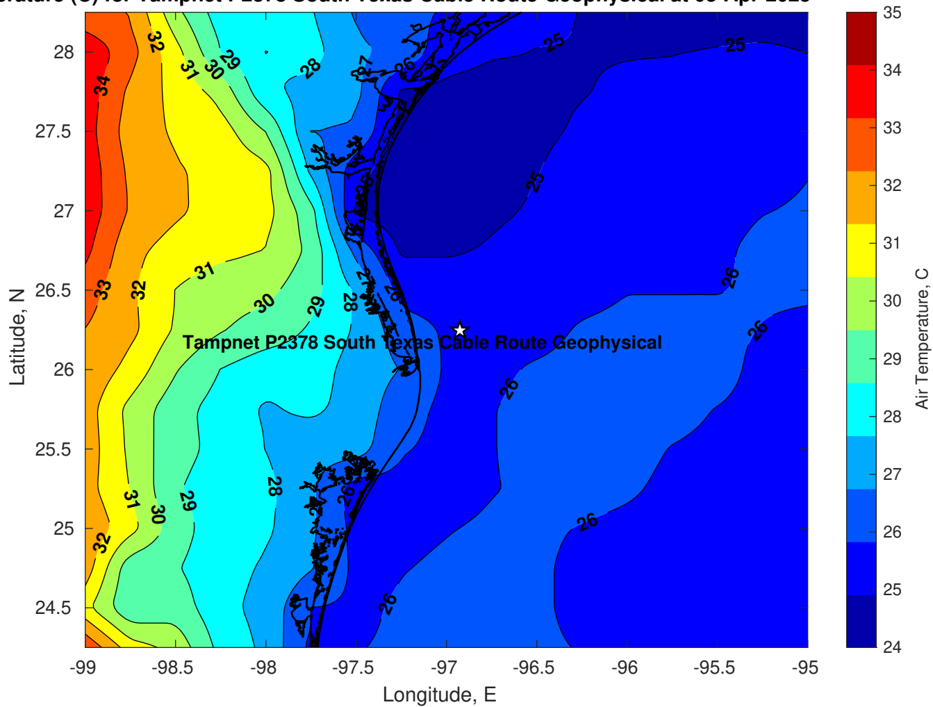
Air Temperature (C) for Tampnet P2378 South Texas Cable Route Geophysical at 03-Apr-2025
