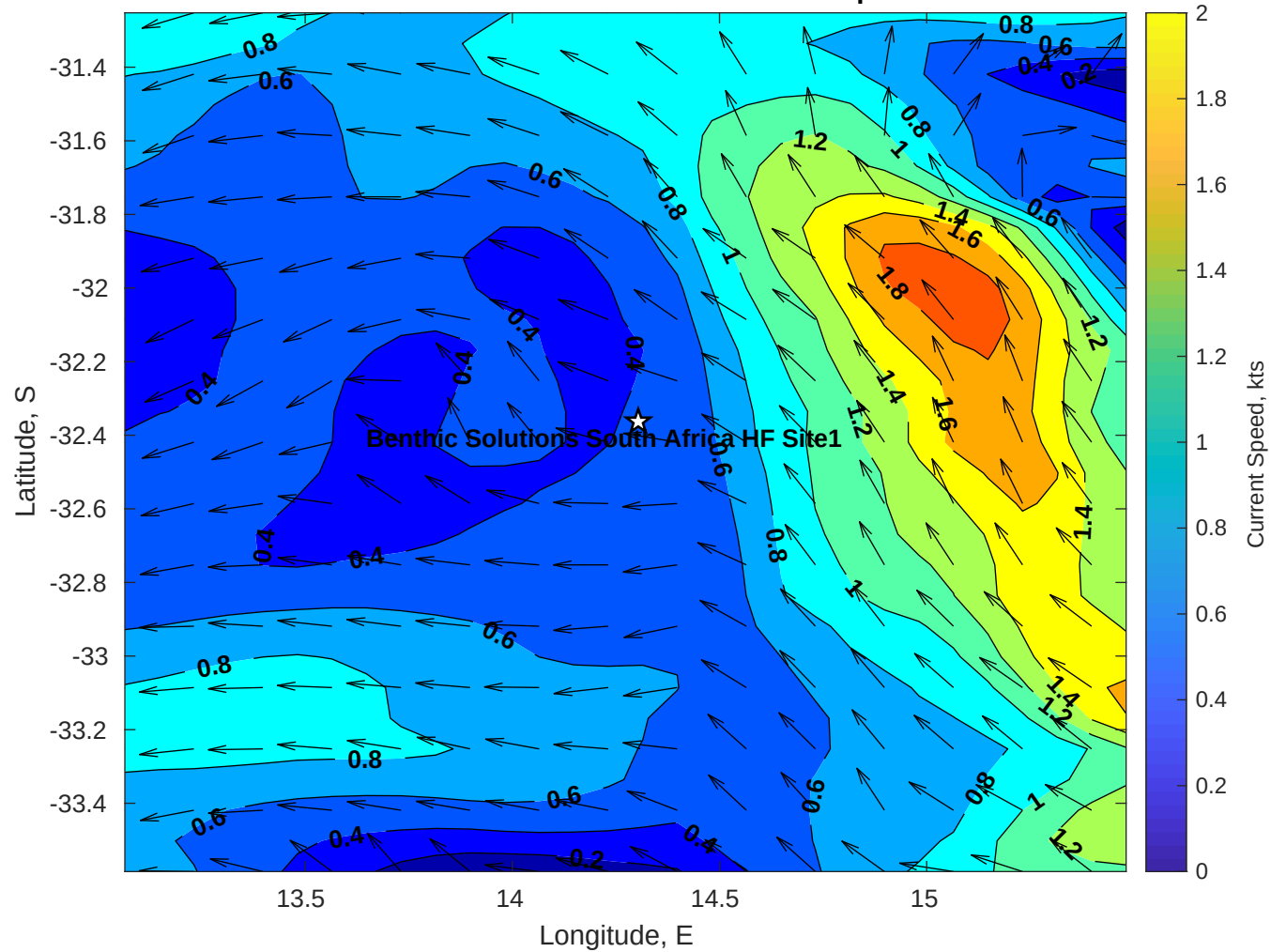
Surface Currents for Benthic Solutions South Africa HF Site1 at 03-Apr-2025 00:00:00
