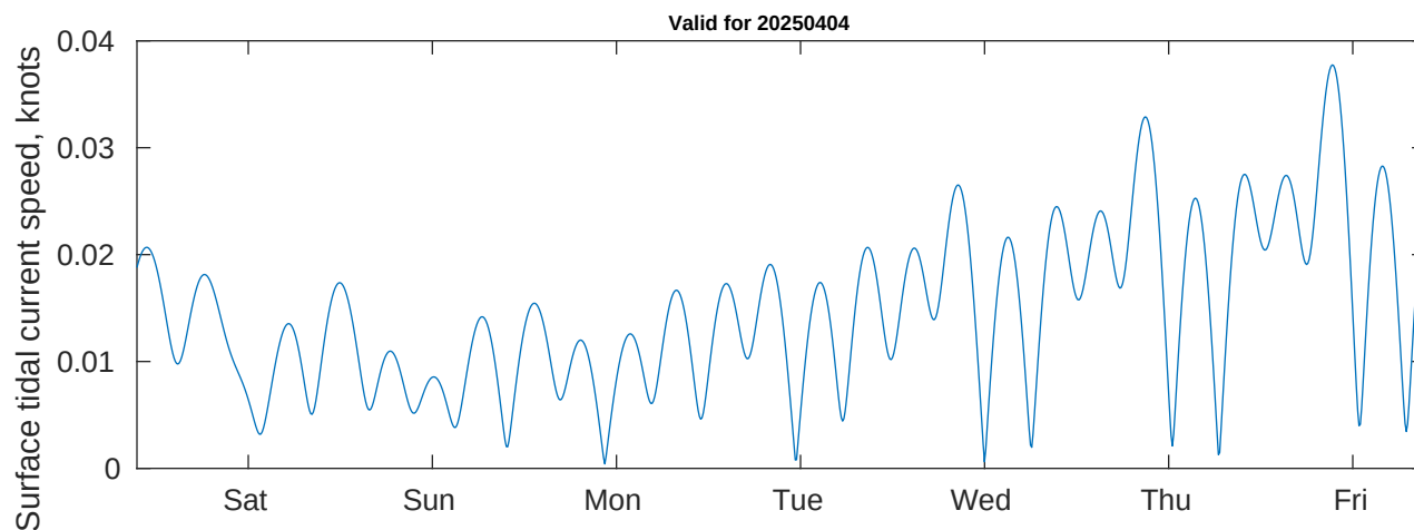
Tidal Currents and Heights for Benthic Solutions South Africa HF Site1 at 20250404
