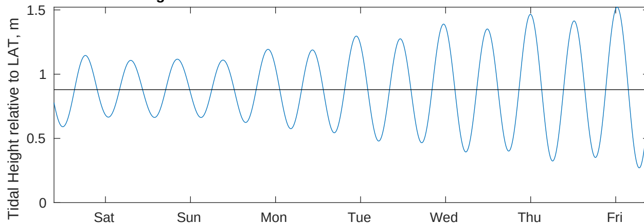
Tidal Currents and Heights for Benthic Solutions South Africa HF Site1 at 20250404
