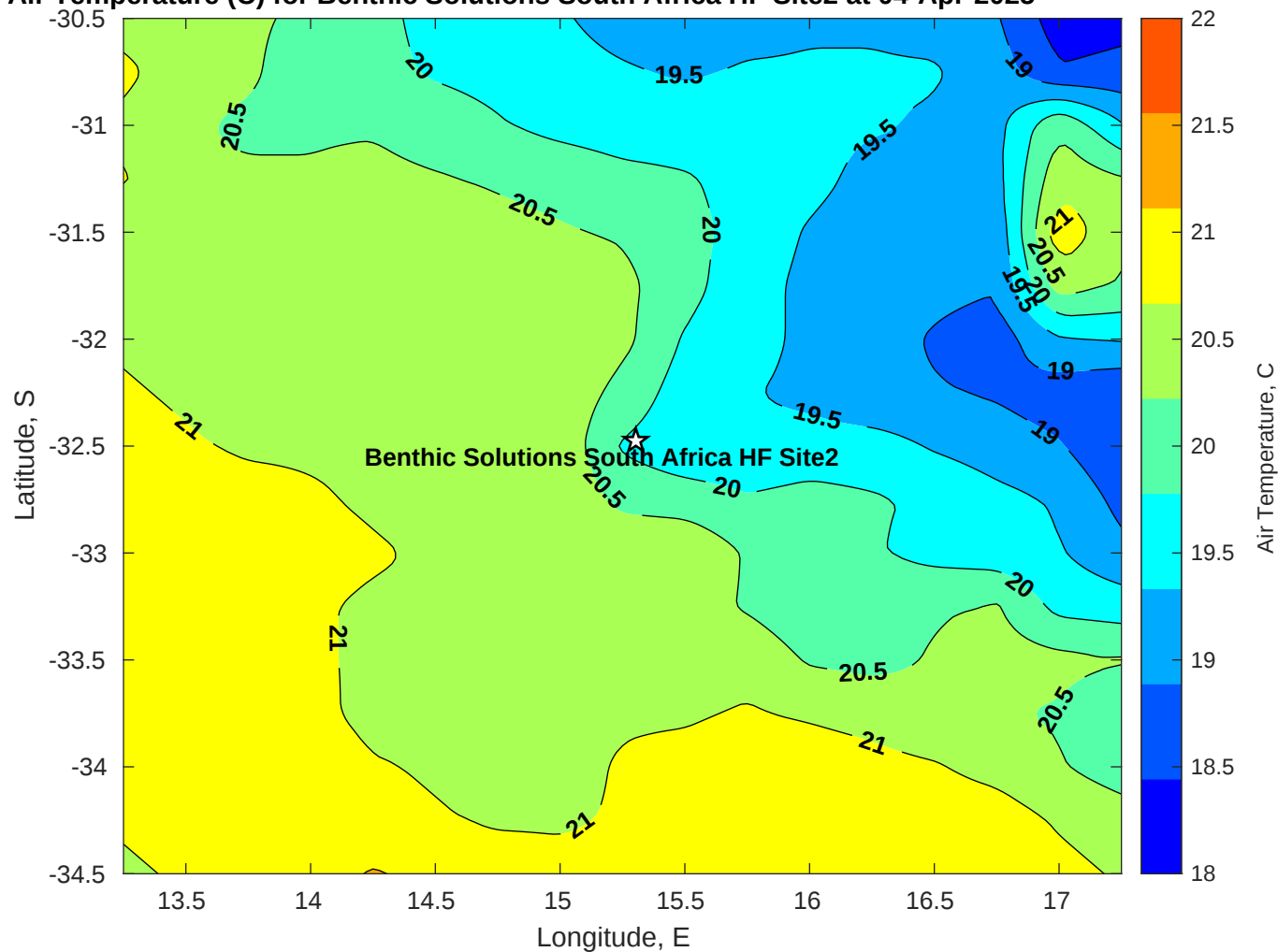
Air Temperature (C) for Benthic Solutions South Africa HF Site2 at 04-Apr-2025
