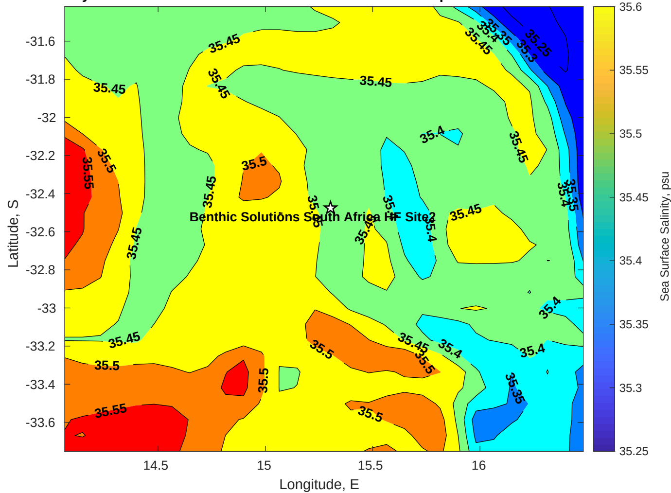
Surface Salinity for Benthic Solutions South Africa HF Site2 at 03-Apr-2025 00:00:00
