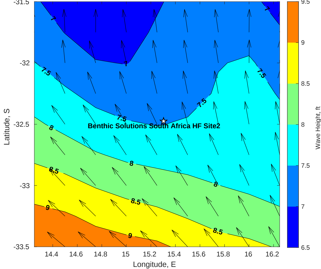
Wave Height (ft) for Benthic Solutions South Africa HF Site2 at 04-Apr-2025 09:00:00
