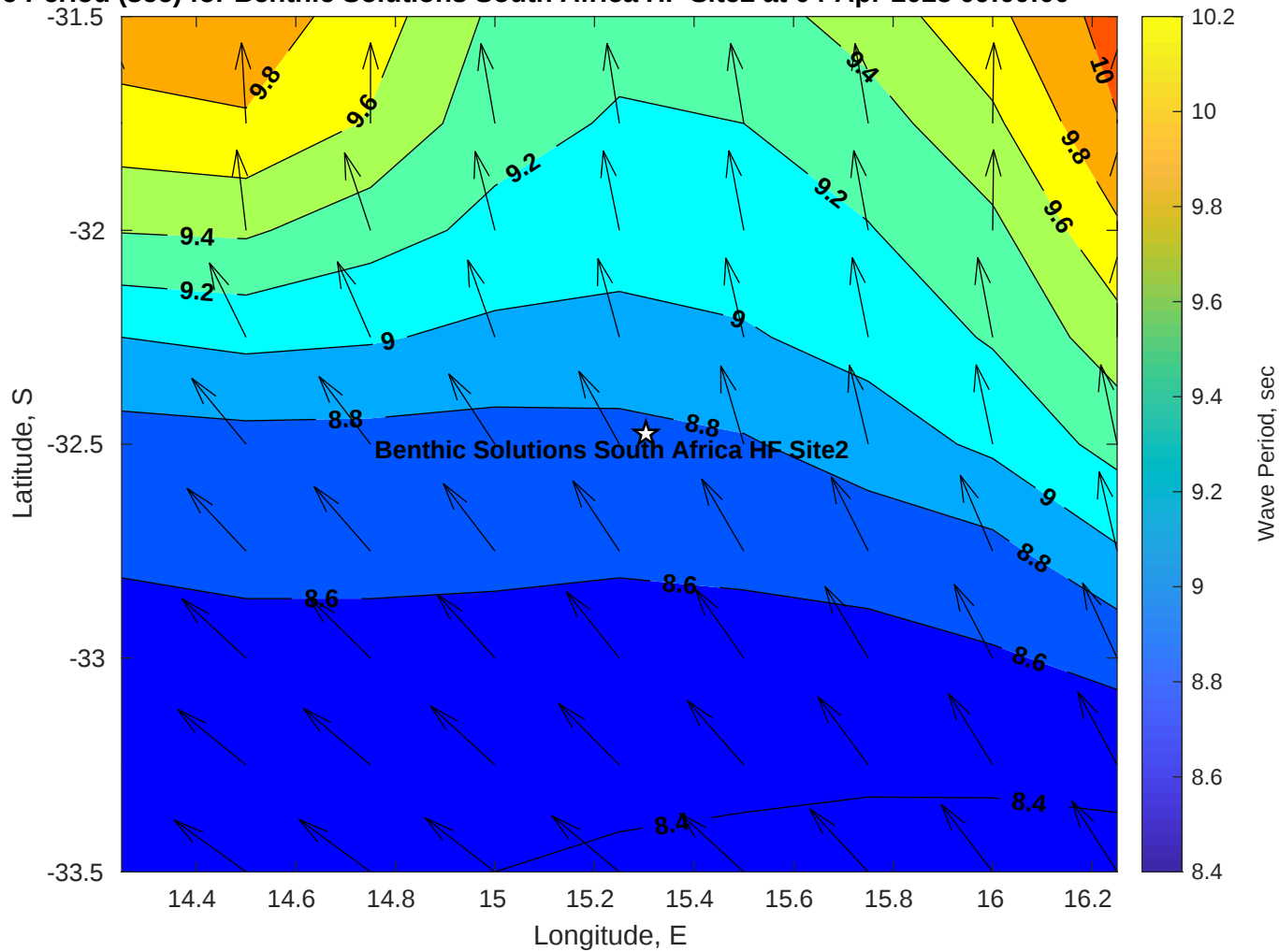
Wave Period (sec) for Benthic Solutions South Africa HF Site2 at 04-Apr-2025 09:00:00
