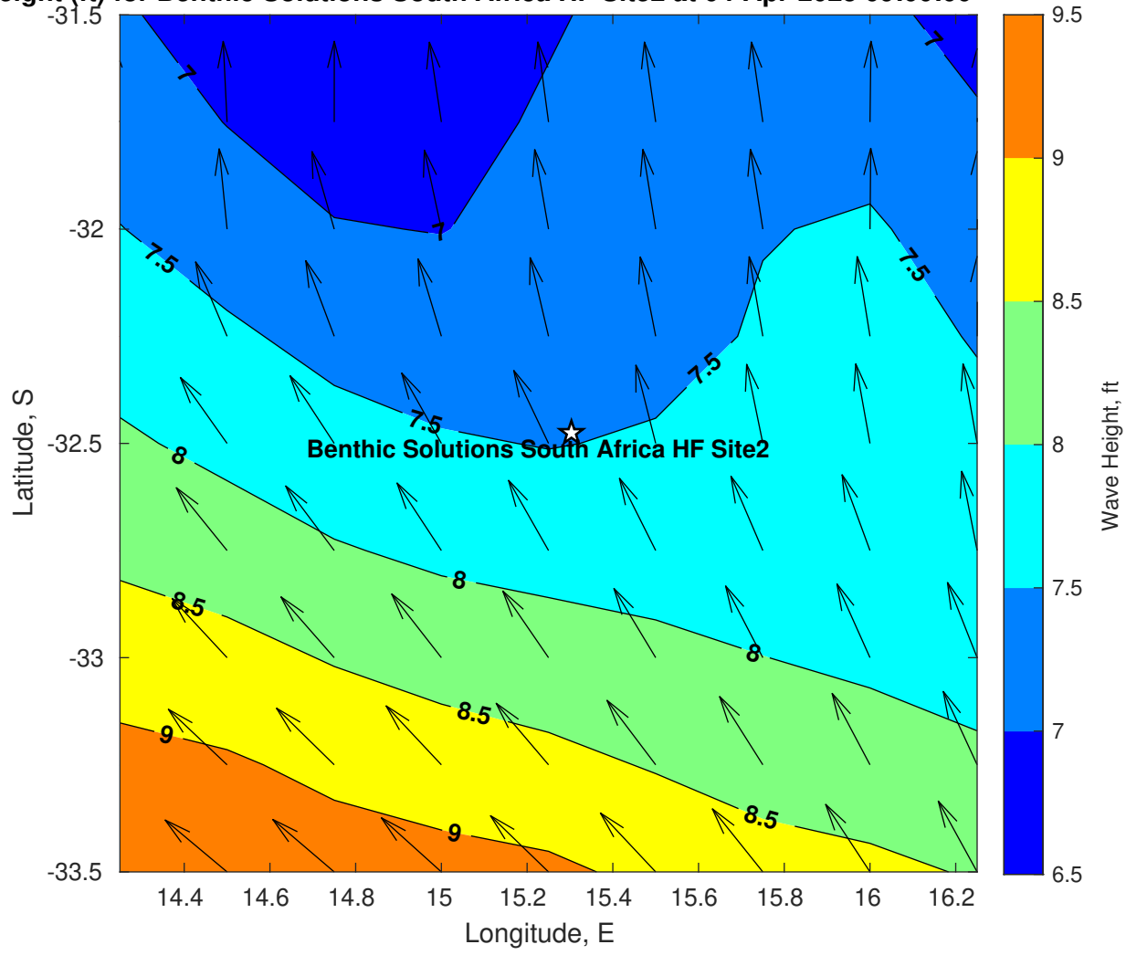
Wave Height (ft) for Benthic Solutions South Africa HF Site2 at 04-Apr-2025 09:00:00
