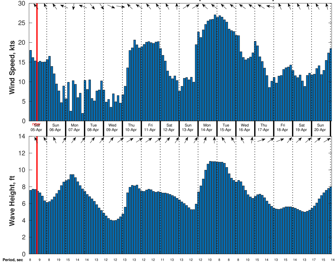
Wind & Wave Forecast for Benthic Solutions South Africa HF Site2 from 04-Apr-2025 02:00:00 to 20-Apr-2025 02:00:00
