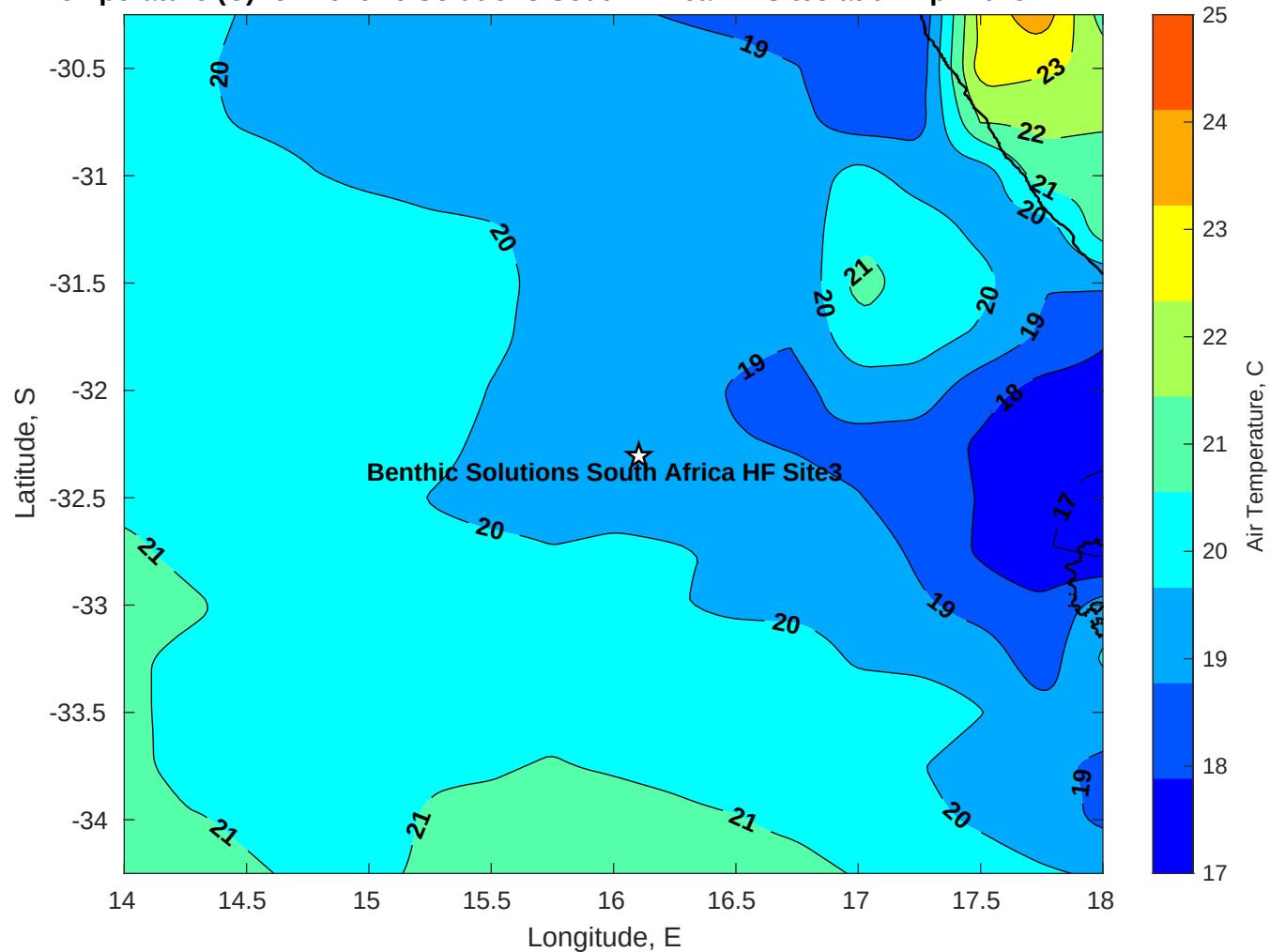
Air Temperature (C) for Benthic Solutions South Africa HF Site3 at 04-Apr-2025
