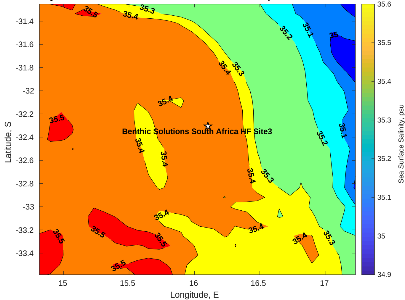
Surface Salinity for Benthic Solutions South Africa HF Site3 at 03-Apr-2025 00:00:00
