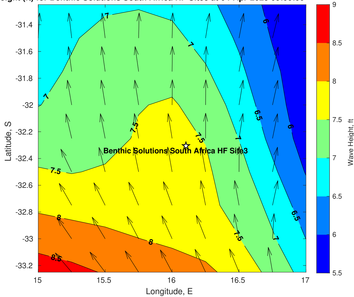
Wave Height (ft) for Benthic Solutions South Africa HF Site3 at 04-Apr-2025 09:00:00
