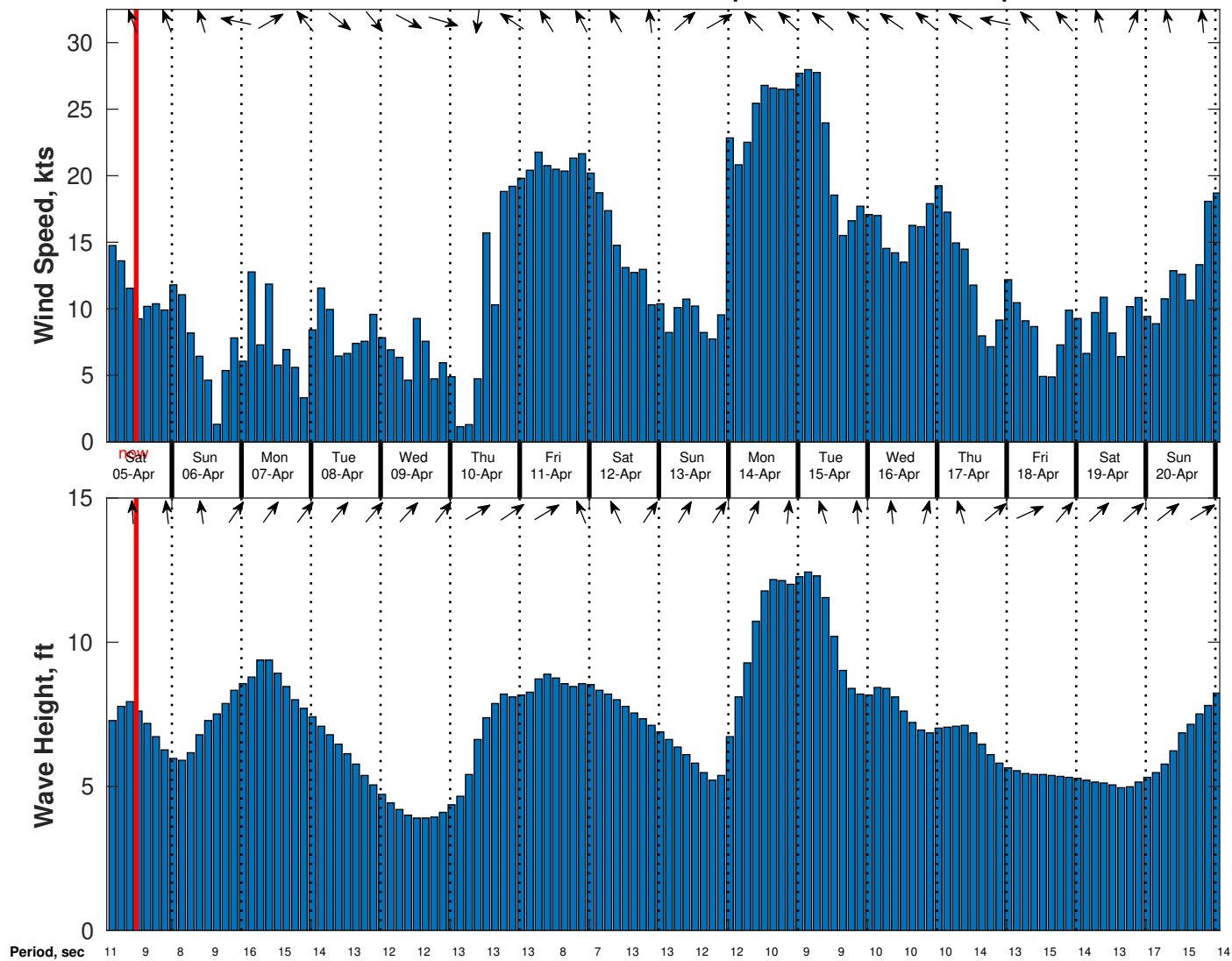
Wind & Wave Forecast for Benthic Solutions South Africa HF Site3 from 04-Apr-2025 02:00:00 to 20-Apr-2025 02:00:00
