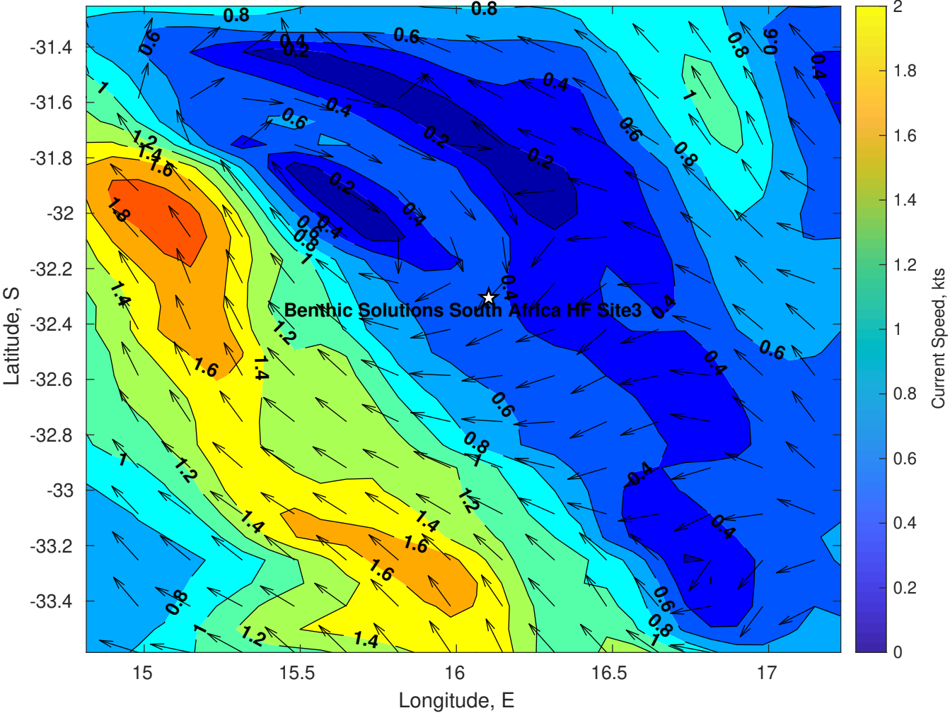
Surface Currents for Benthic Solutions South Africa HF Site3 at 03-Apr-2025 00:00:00
