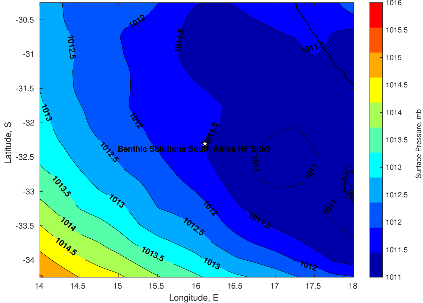
Surface Pressure (mb) for Benthic Solutions South Africa HF Site3 at 05-Apr-2025 00:00:00
