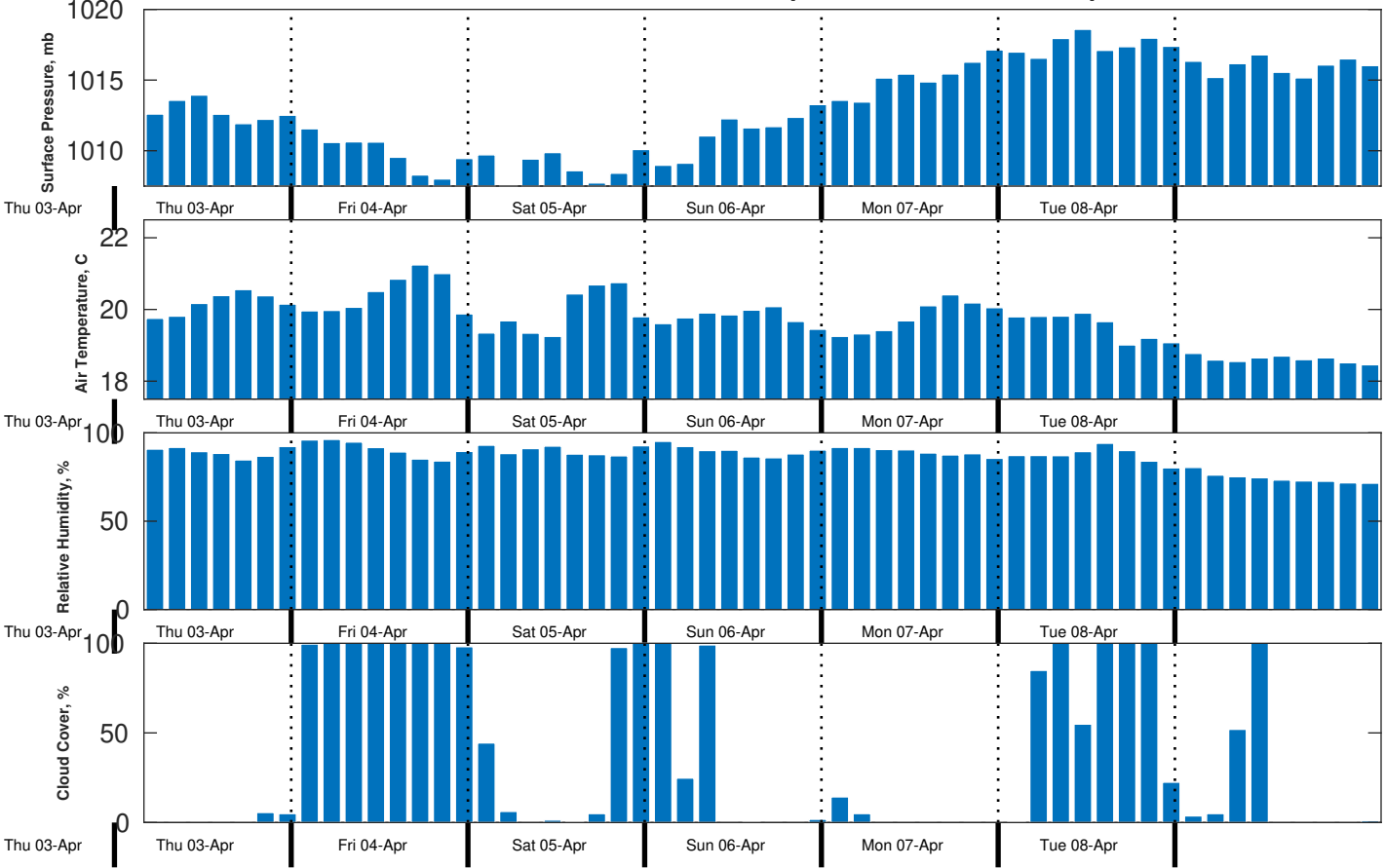
Met Forecast for Benthic Solutions South Africa HF Site3 from 04-Apr-2025 00:00:00 to 11-Apr-2025 00:00:00
