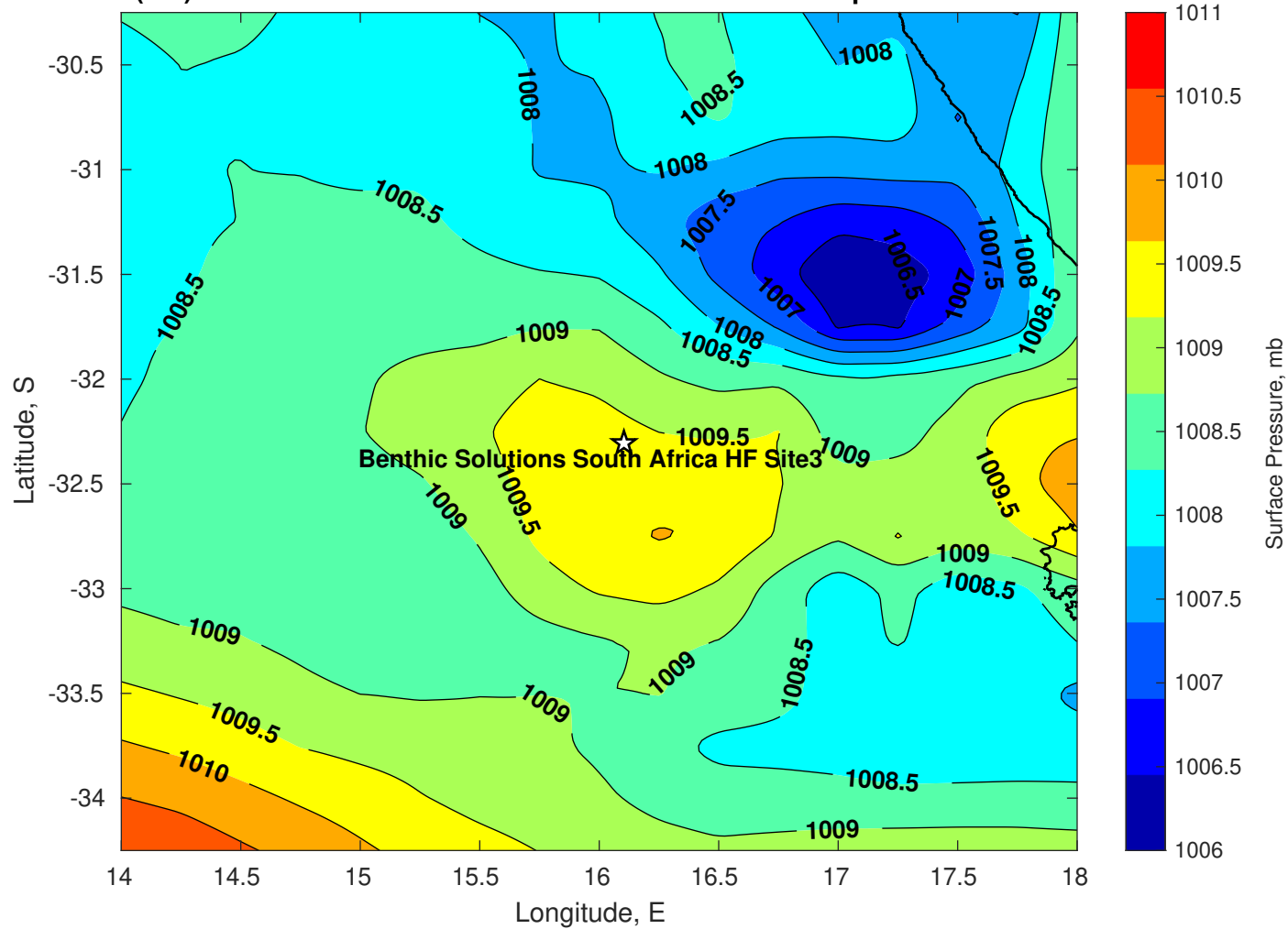
Surface Pressure (mb) for Benthic Solutions South Africa HF Site3 at 06-Apr-2025 00:00:00
