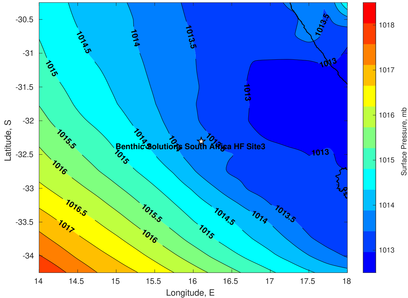
Surface Pressure (mb) for Benthic Solutions South Africa HF Site3 at 04-Apr-2025 00:00:00
