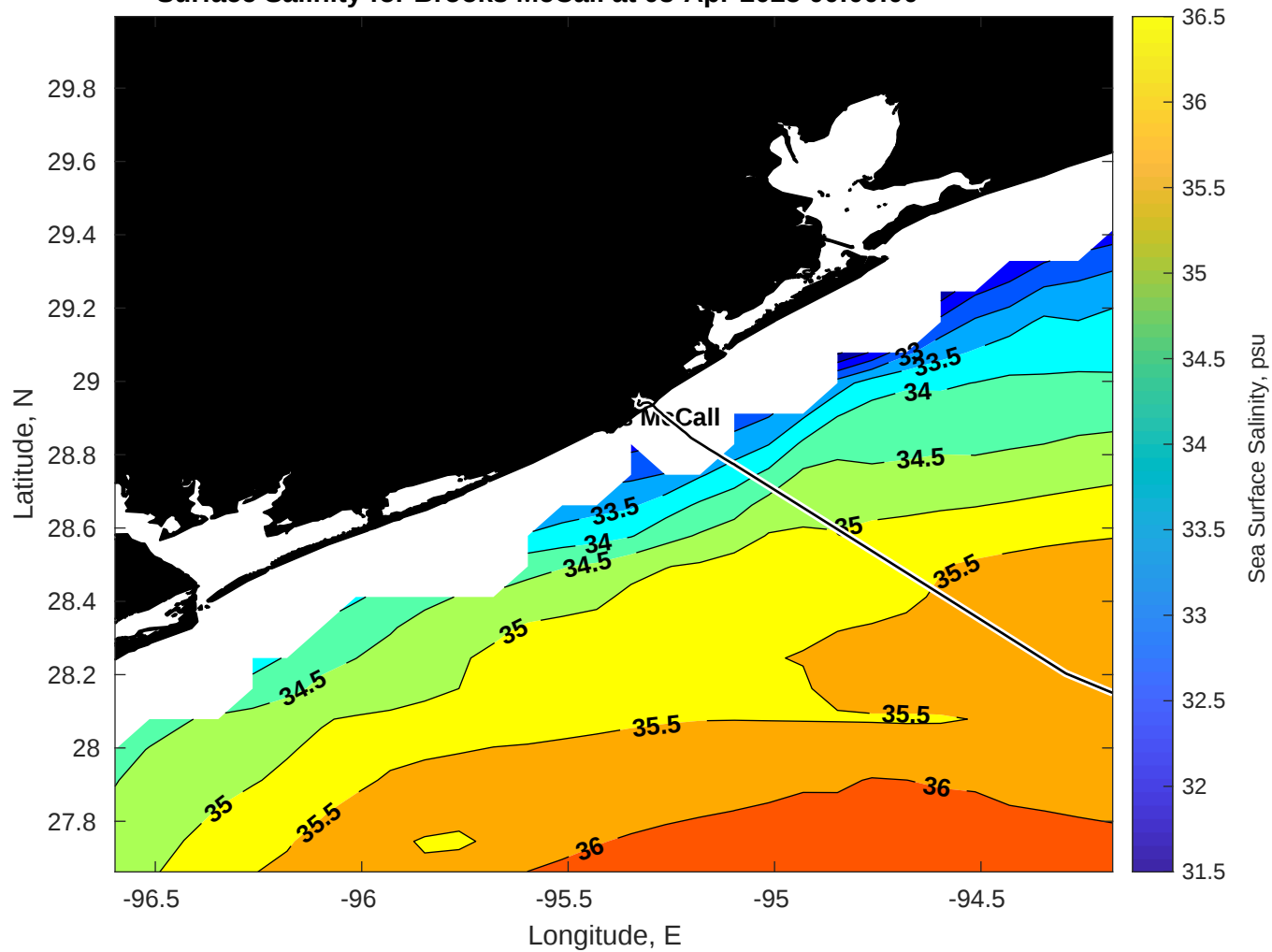
Surface Salinity for Brooks McCall at 03-Apr-2025 00:00:00
