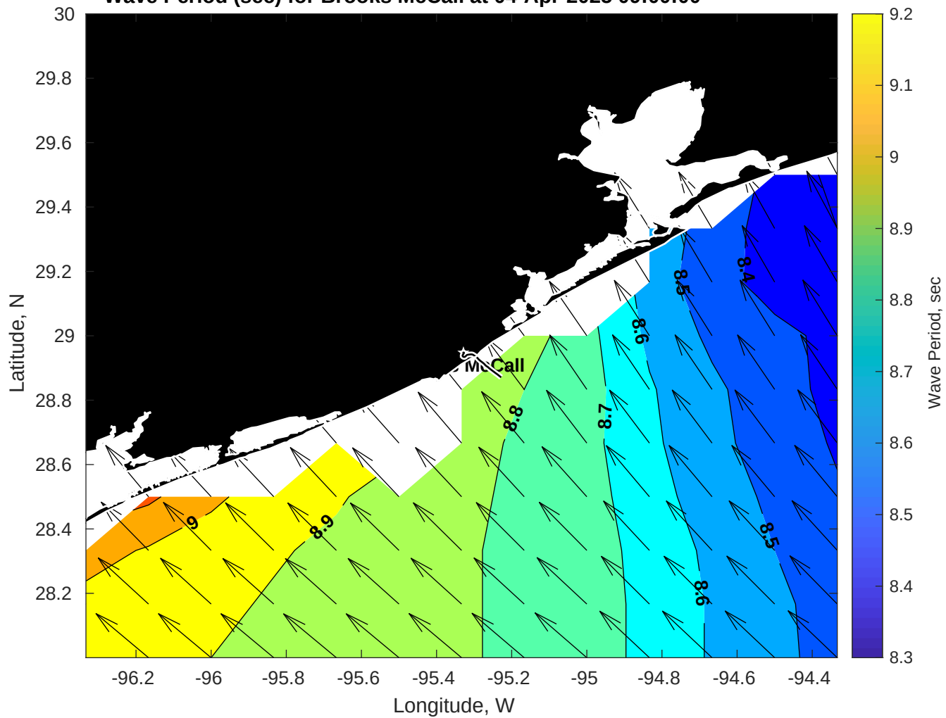
Wave Period (sec) for Brooks McCall at 04-Apr-2025 09:00:00
