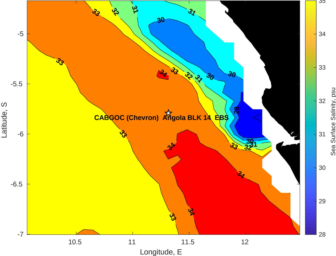
Surface Salinity for CABGOC (Chevron) Angola BLK 14 EBS at 03-Apr-2025 00:00:00
