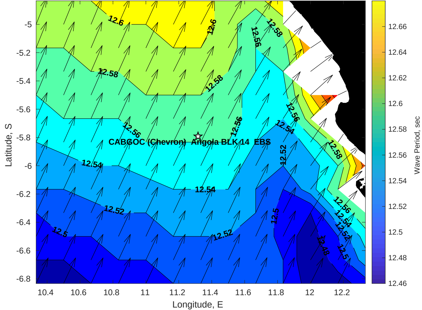
Wave Period (sec) for CABGOC (Chevron) Angola BLK 14 EBS at 04-Apr-2025 09:00:00
