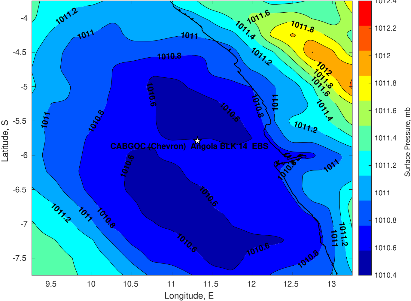
Surface Pressure (mb) for CABGOC (Chevron) Angola BLK 14 EBS at 04-Apr-2025 00:00:00
