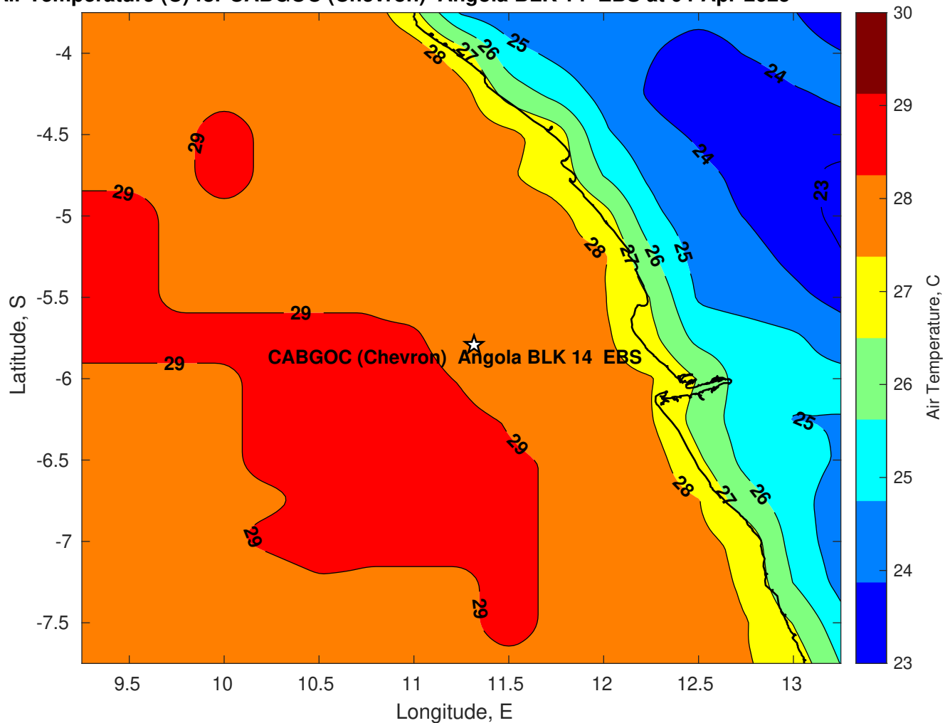
Air Temperature (C) for CABGOC (Chevron) Angola BLK 14 EBS at 04-Apr-2025
