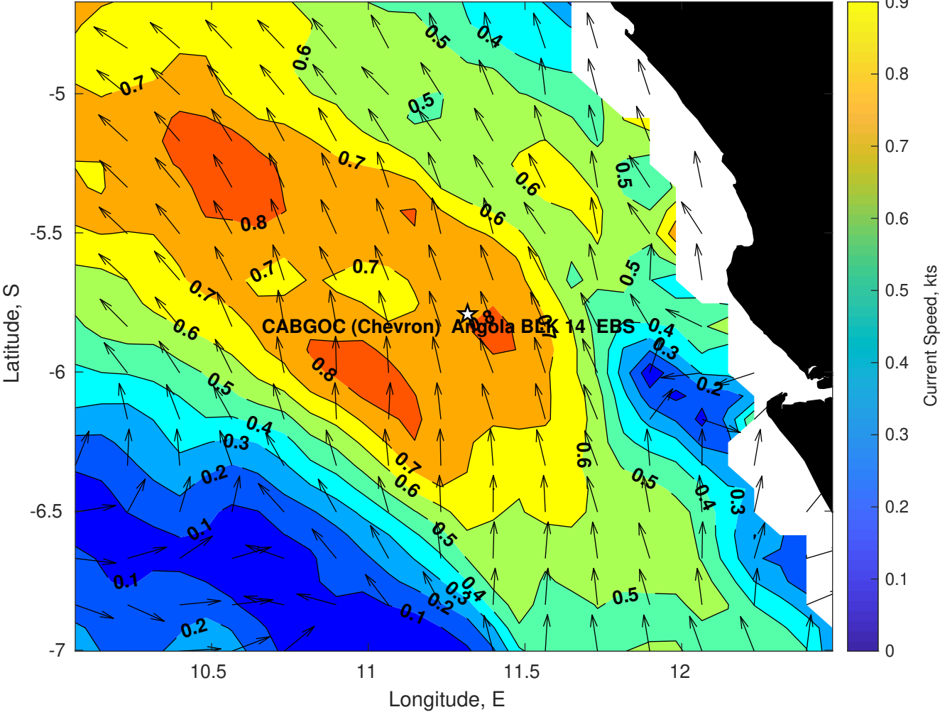
Surface Currents for CABGOC (Chevron) Angola BLK 14 EBS at 03-Apr-2025 00:00:00
