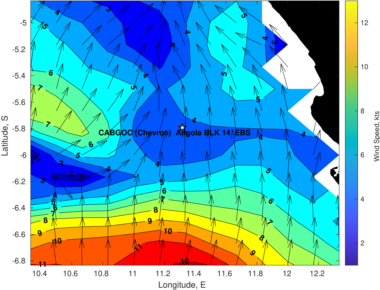
Winds (kts) for CABGOC (Chevron) Angola BLK 14 EBS at 04-Apr-2025 09:00:00
