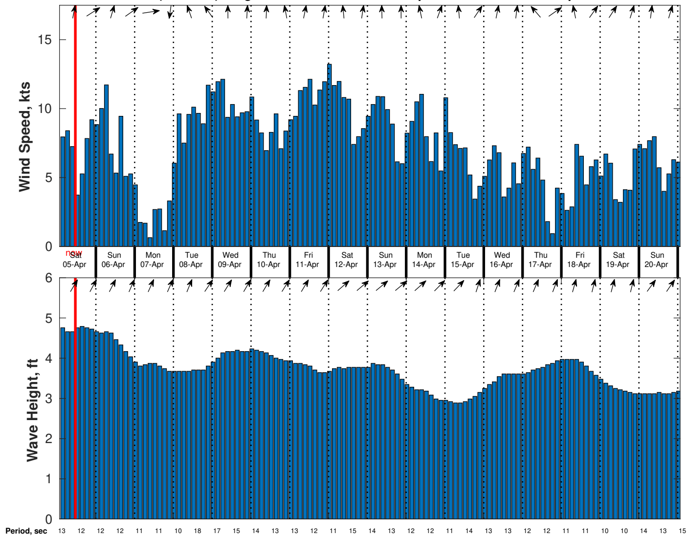
Wind & Wave Forecast for CABGOC (Chevron) Angola BLK 14 EBS from 04-Apr-2025 02:00:00 to 20-Apr-2025 02:00:00
