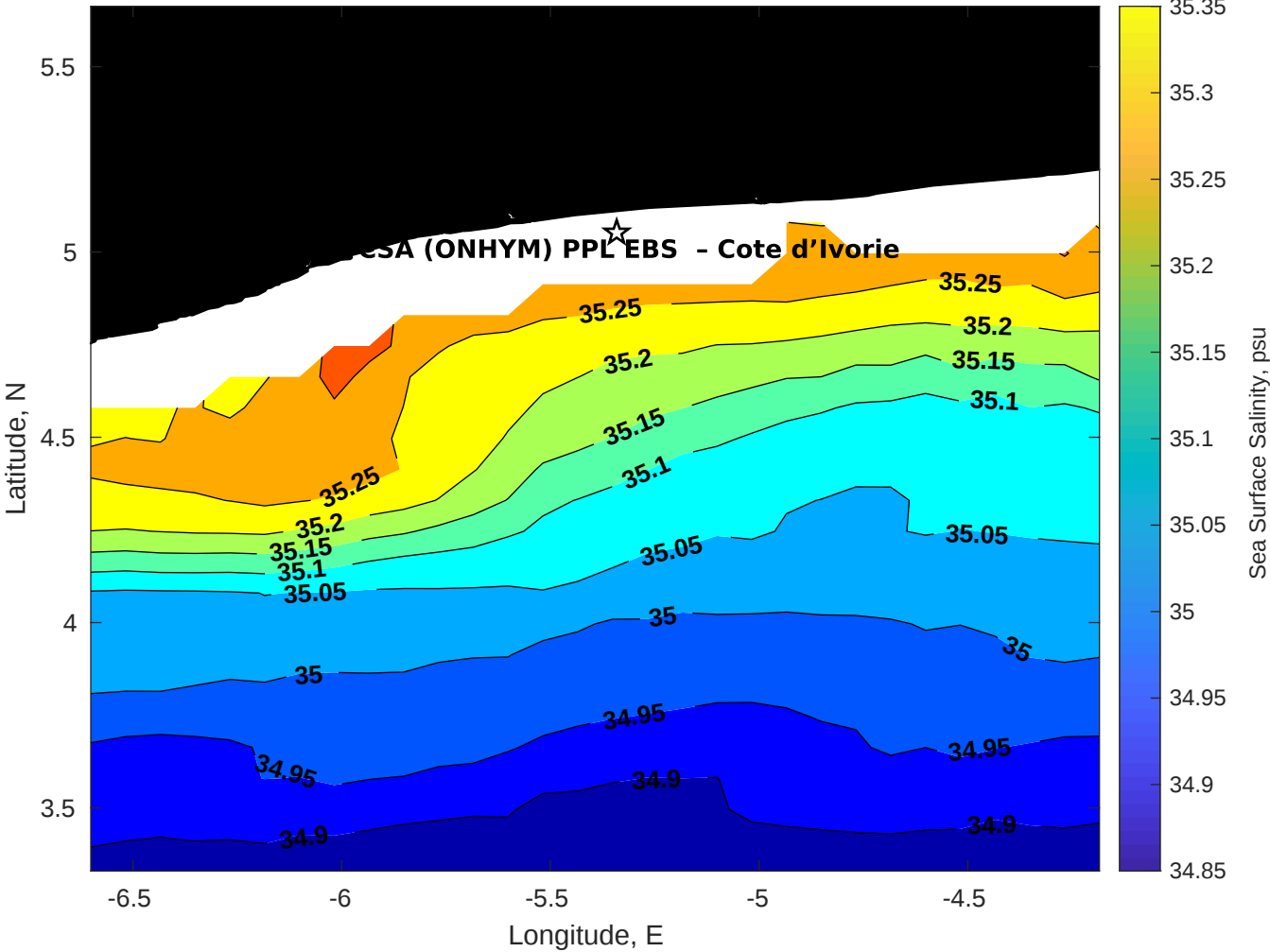
Surface Salinity for CSA (ONHYM) PPL EBS - Cote d'Ivoire at 03-Apr-2025 00:00:00
