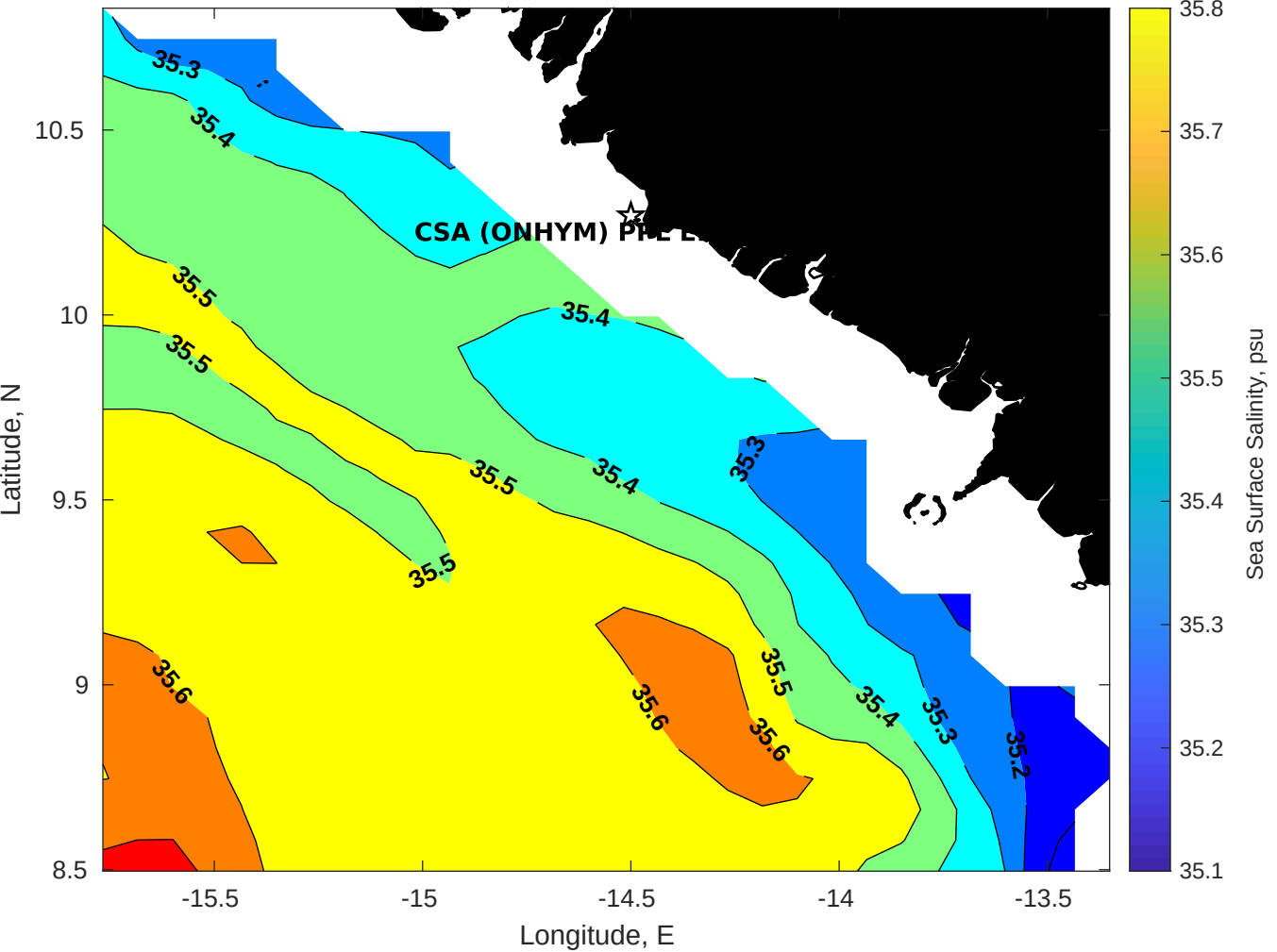
Surface Salinity for CSA (ONHYM) PPL EBS - Guinea at 03-Apr-2025 00:00:00
