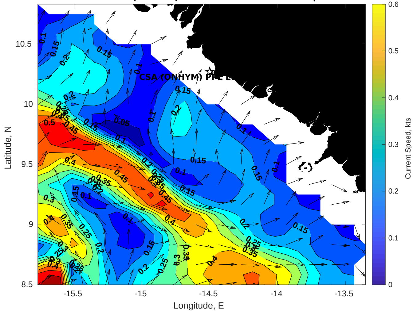
Surface Currents for CSA (ONHYM) PPL EBS - Guinea at 03-Apr-2025 00:00:00
