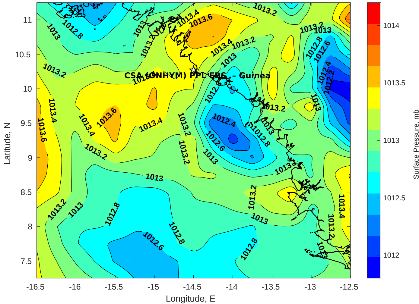
Surface Pressure (mb) for CSA (ONHYM) PPL EBS - Guinea at 04-Apr-2025 00:00:00
