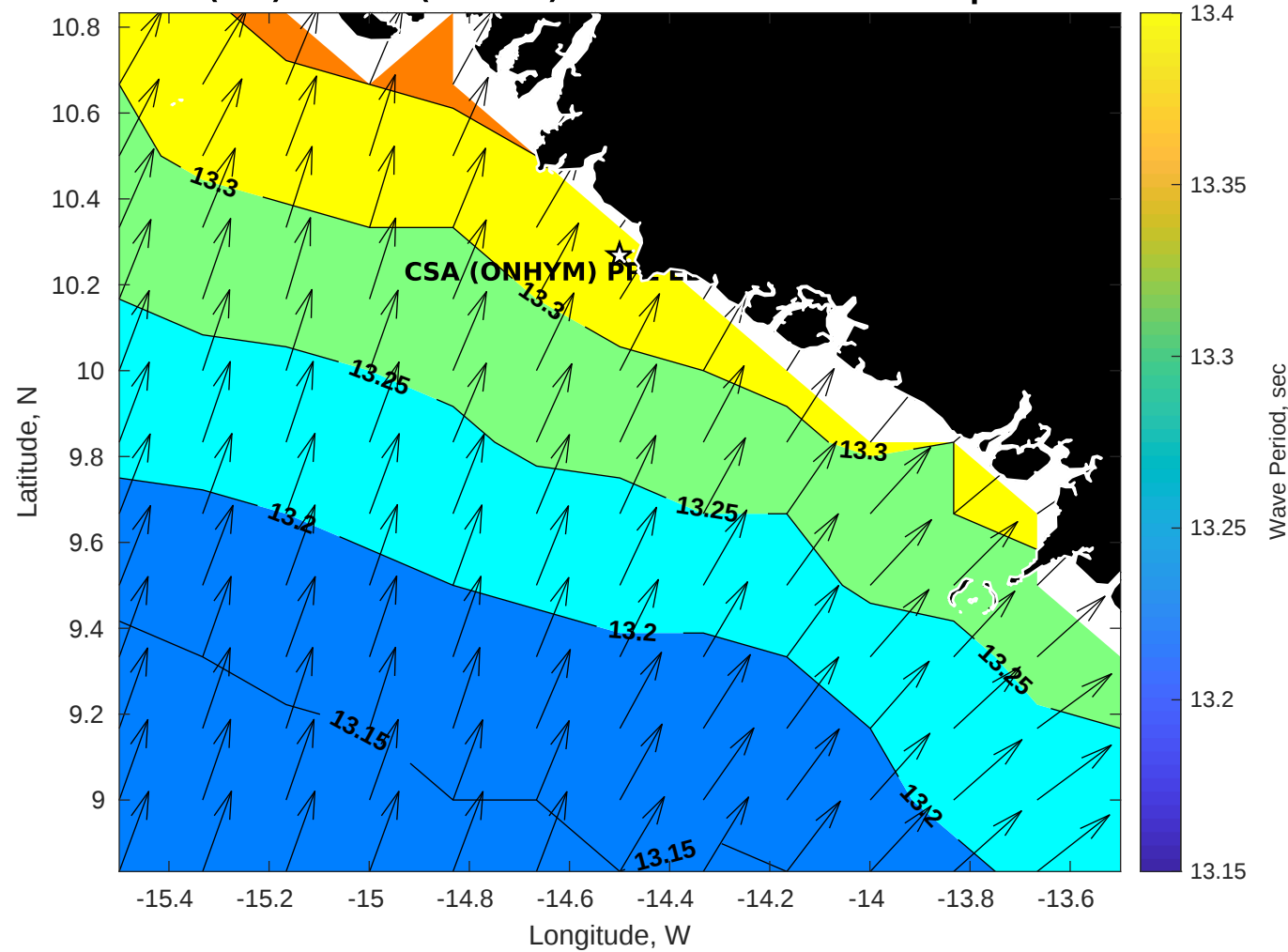
Wave Period (sec) for CSA (ONHYM) PPL EBS - Guinea at 04-Apr-2025 09:00:00
