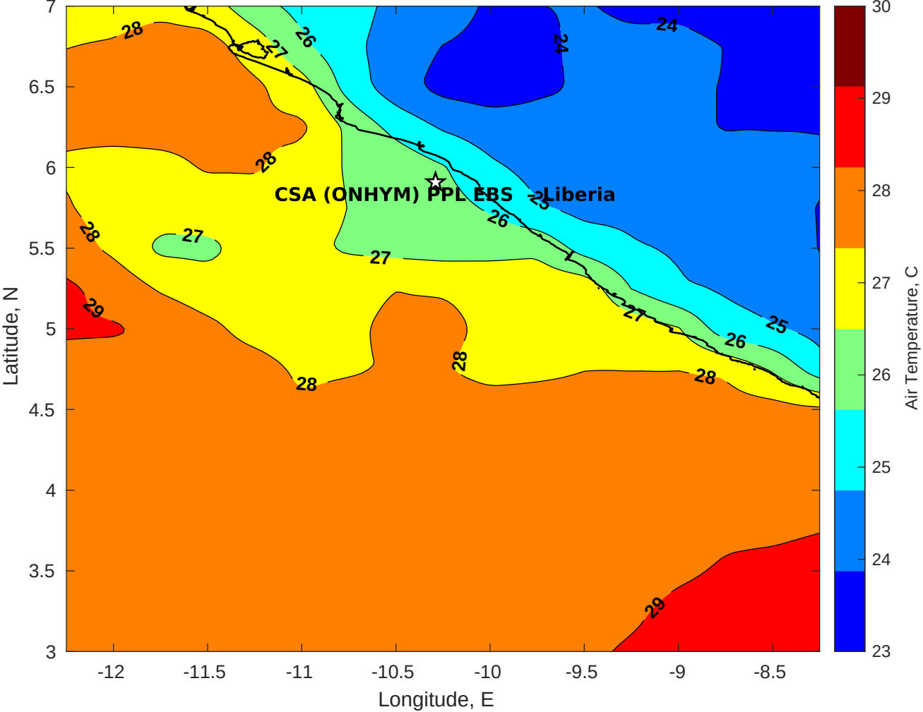
Air Temperature (C) for CSA (ONHYM) PPL EBS - Liberia at 04-Apr-2025
