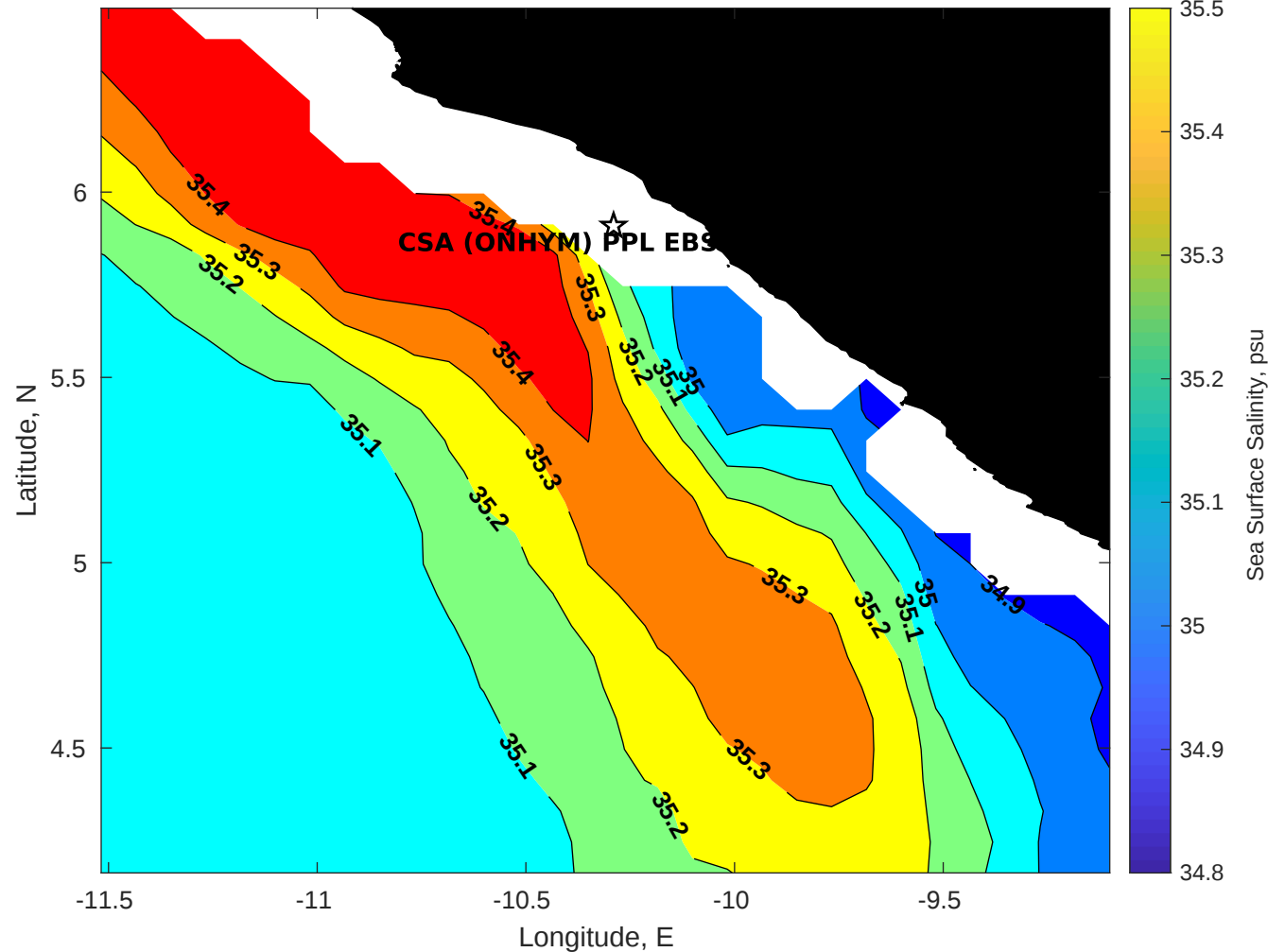
Surface Salinity for CSA (ONHYM) PPL EBS - Liberia at 03-Apr-2025 00:00:00
