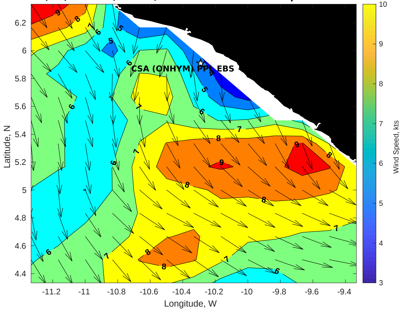
Winds (kts) for CSA (ONHYM) PPL EBS - Liberia at 04-Apr-2025 09:00:00
