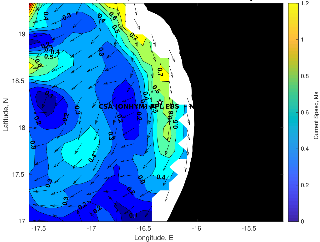
Surface Currents for CSA (ONHYM) PPL EBS - Mauritania at 03-Apr-2025 00:00:00
