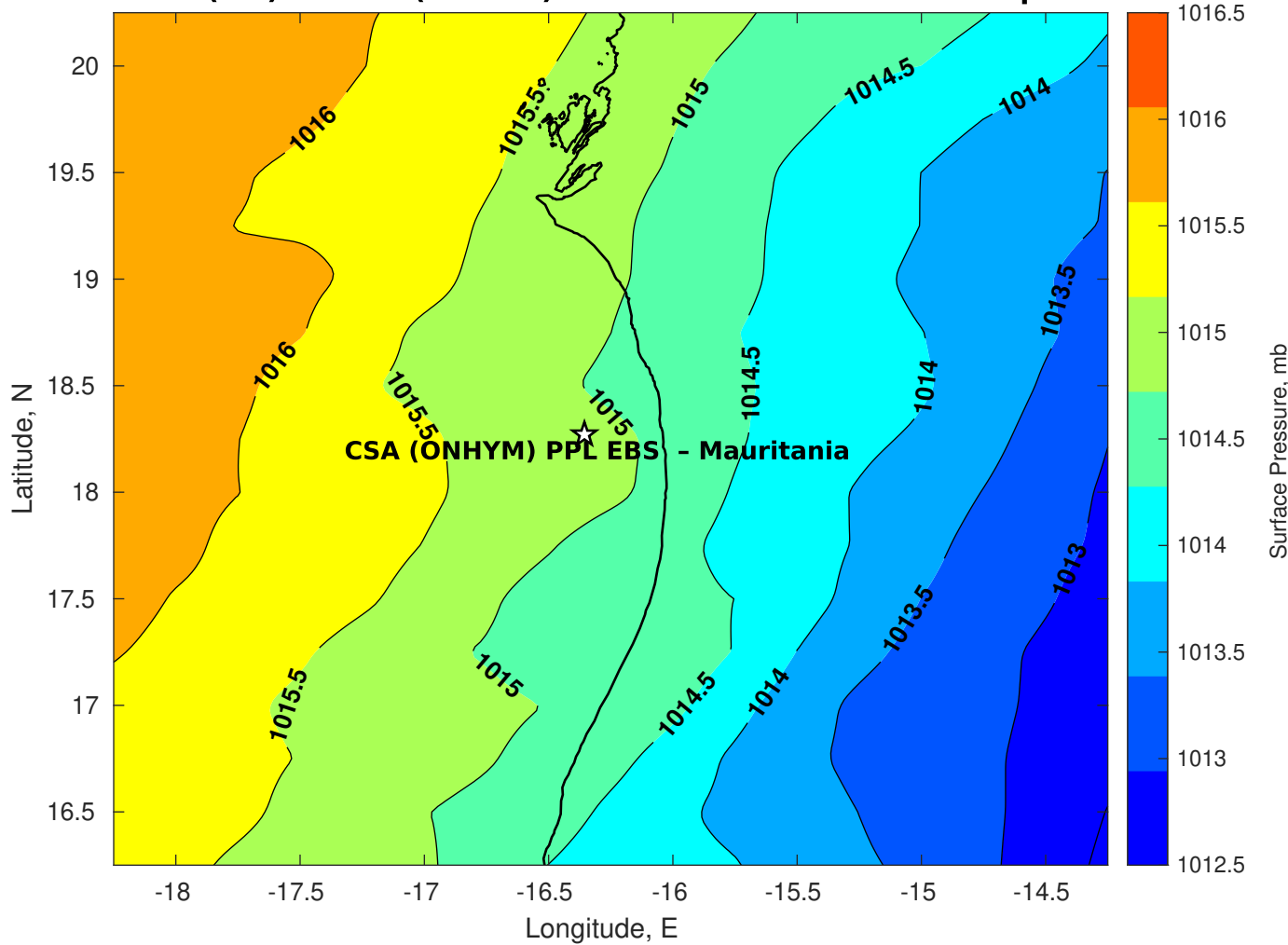
Surface Pressure (mb) for CSA (ONHYM) PPL EBS - Mauritania at 04-Apr-2025 00:00:00
