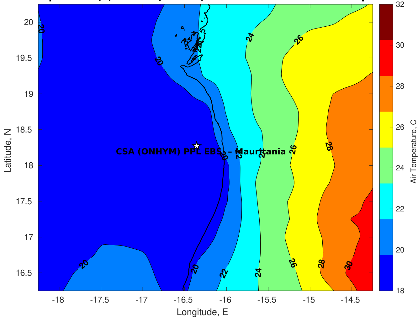
Air Temperature (C) for CSA (ONHYM) PPL EBS - Mauritania at 04-Apr-2025
