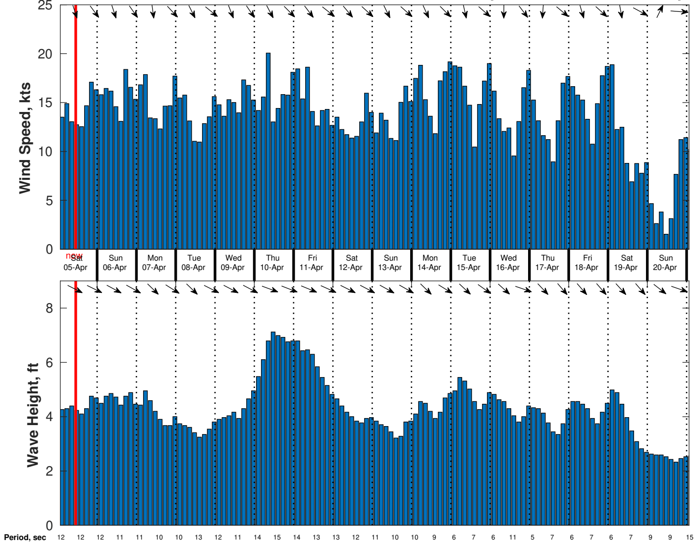
Wind & Wave Forecast for CSA (ONHYM) PPL EBS - Mauritania from 04-Apr-2025 01:00:00 to 20-Apr-2025 01:00:00
