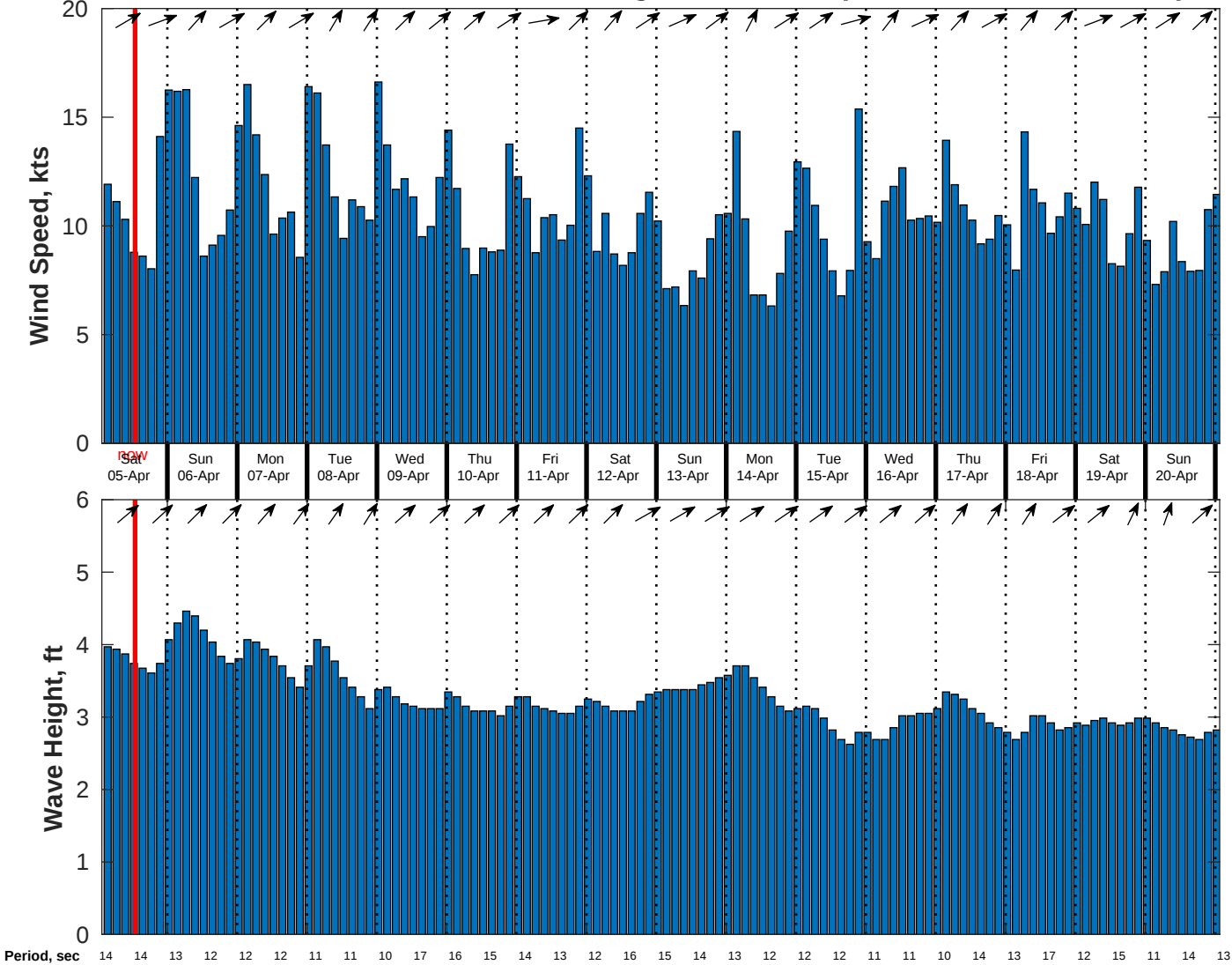
Wind & Wave Forecast for CSA (ONHYM) PPL EBS - Nigeria from 04-Apr-2025 02:00:00 to 20-Apr-2025 02:00:00
