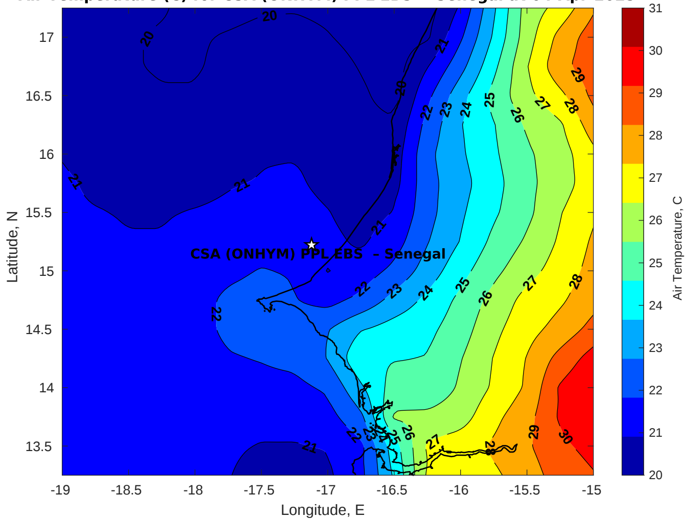
Air Temperature (C) for CSA (ONHYM) PPL EBS - Senegal at 04-Apr-2025
