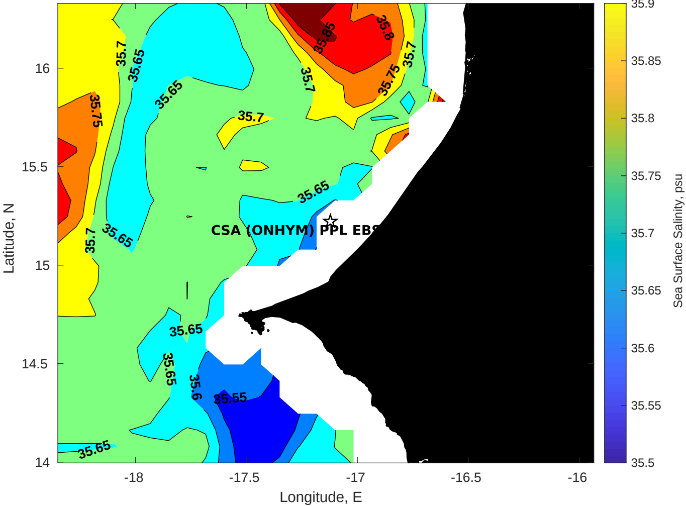
Surface Salinity for CSA (ONHYM) PPL EBS - Senegal at 03-Apr-2025 00:00:00
