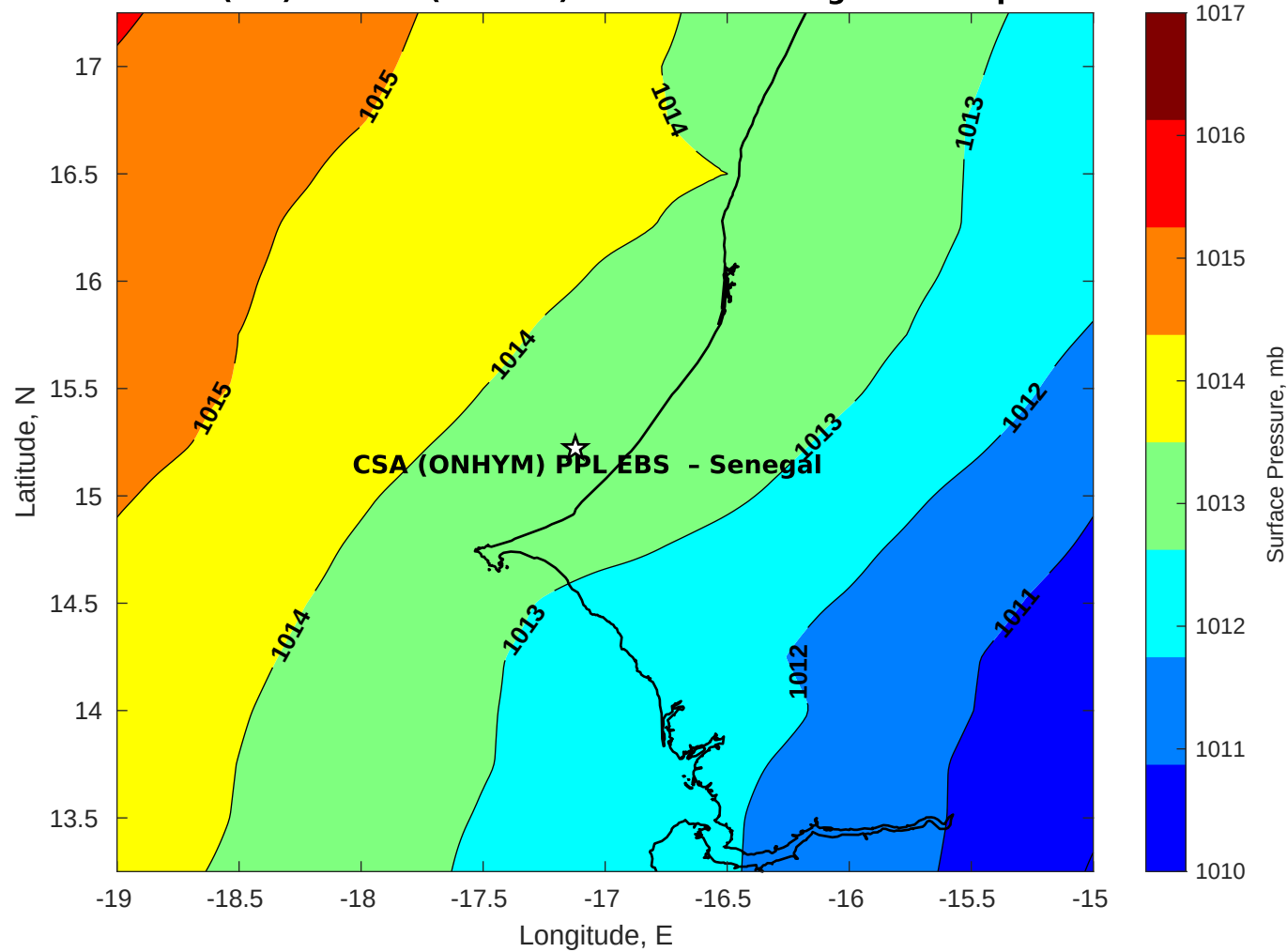
Surface Pressure (mb) for CSA (ONHYM) PPL EBS - Senegal at 05-Apr-2025 00:00:00
