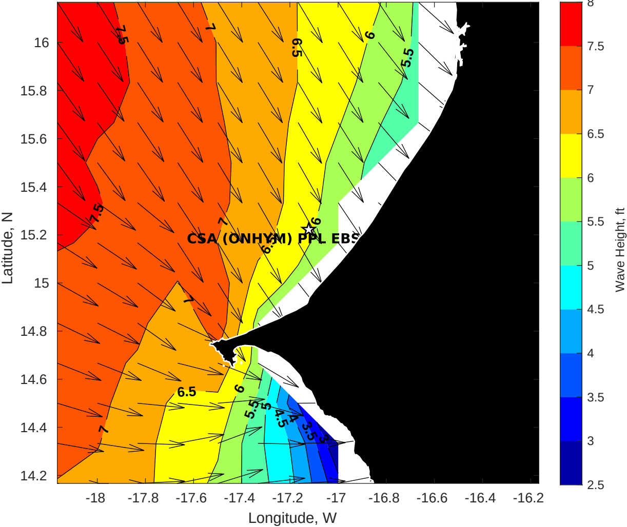
Wave Height (ft) for CSA (ONHYM) PPL EBS - Senegal at 04-Apr-2025 09:00:00
