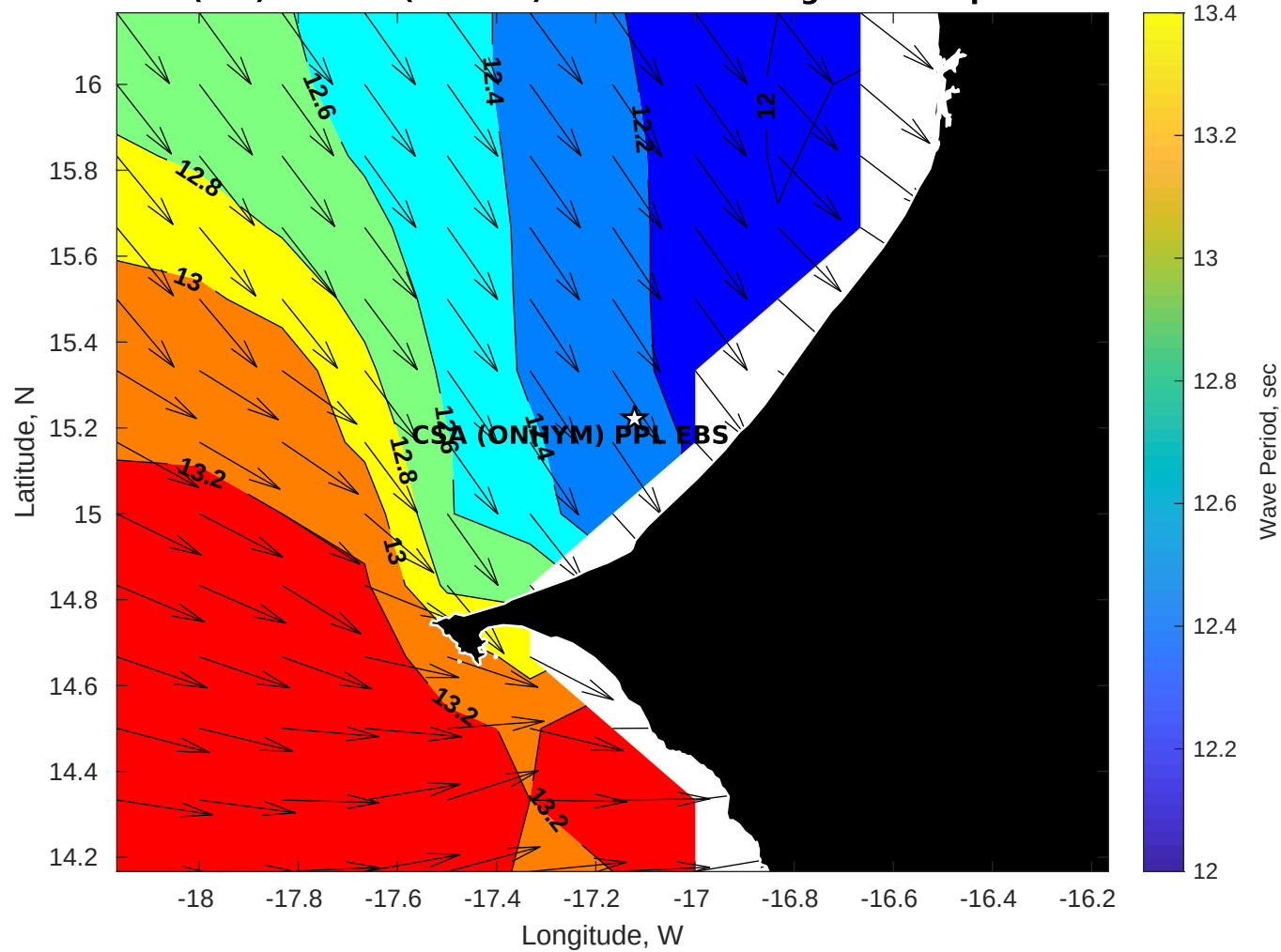
Wave Period (sec) for CSA (ONHYM) PPL EBS - Senegal at 04-Apr-2025 09:00:00
