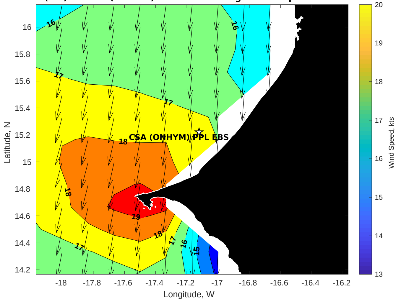
Winds (kts) for CSA (ONHYM) PPL EBS - Senegal at 04-Apr-2025 09:00:00
