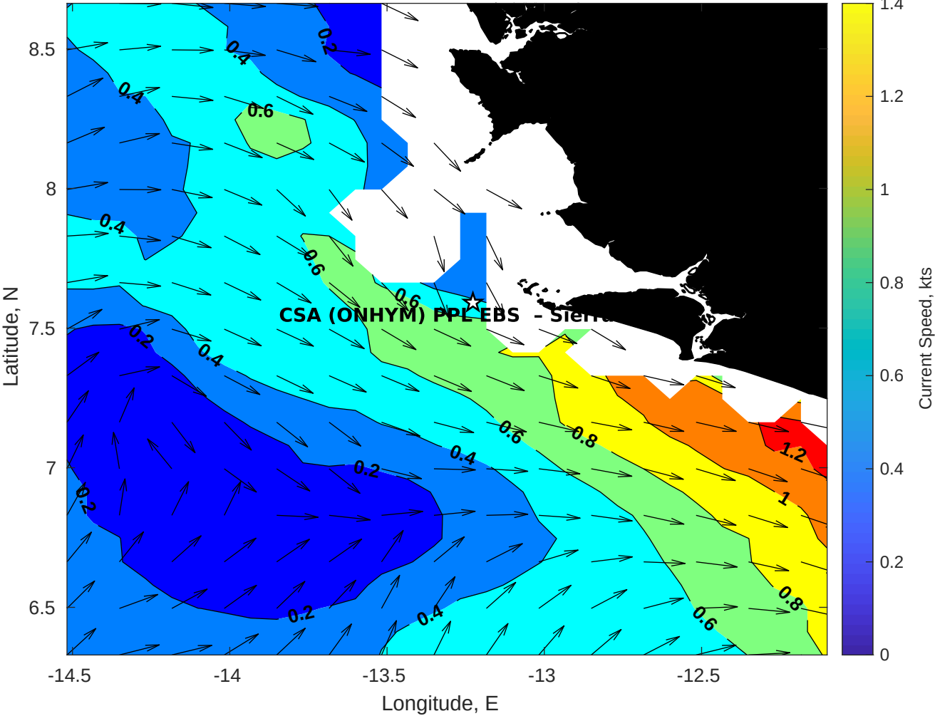
Surface Currents for CSA (ONHYM) PPL EBS - Sierra Leone at 03-Apr-2025 00:00:00
